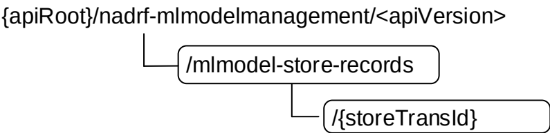
Figure 5.2.3.1-1: Resource URI structure of the Nadrf_MLModelManagement API
