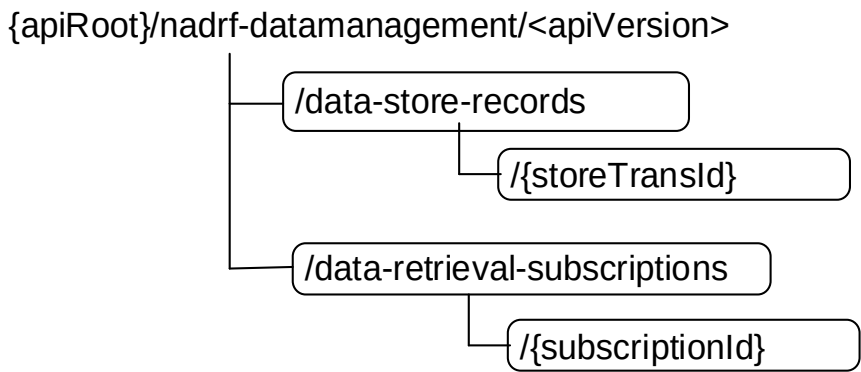
Figure 5.1.3.1-1: Resource URI structure of the Nadrif_DataManagement API
