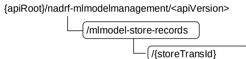
Figure 5.2.3.1-1: Resource URI structure of the Nadrif_MLModelManagement API
