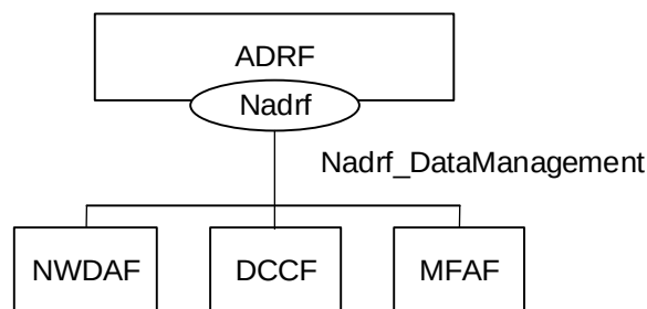
Figure 4.2.1.2-1: Reference Architecture for the Nadrf_DataManagement Service; SBI representation
