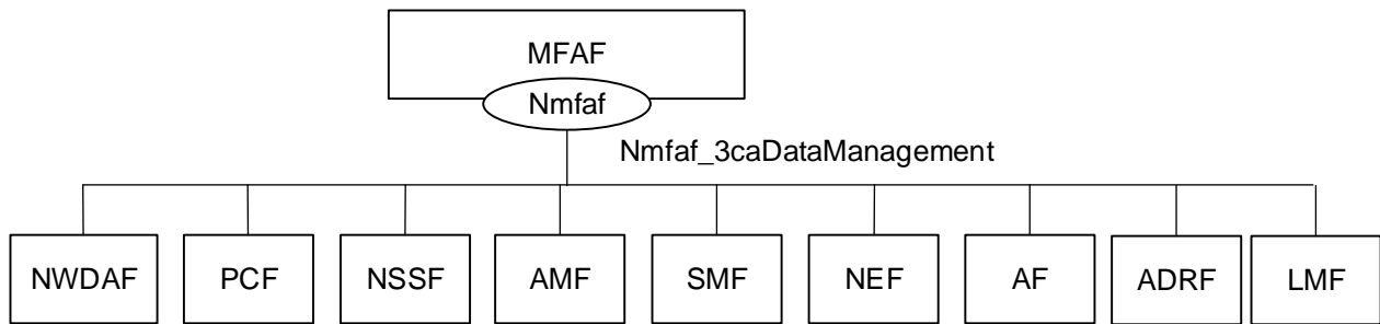
Figure 4.3.1.2-1: Reference Architecture for the Nmfaf_3caDataManagement Service; SBI representation
