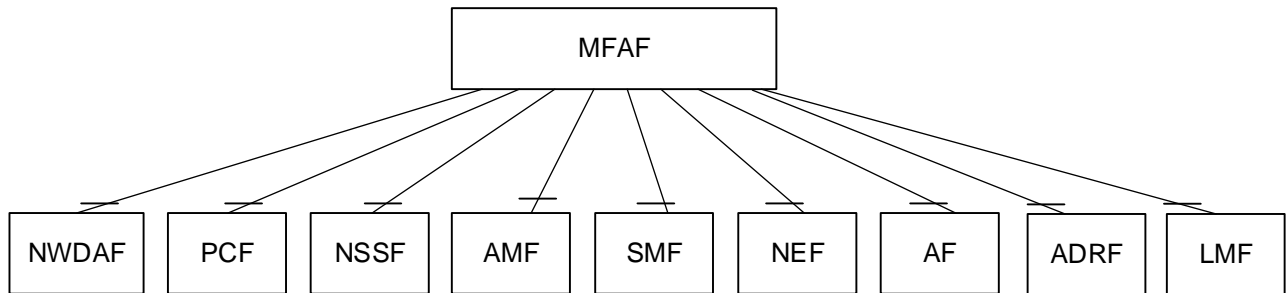
Figure 4.3.1.2-2: Reference Architecture for the Nmfaf_3caDataManagement Service; reference point
