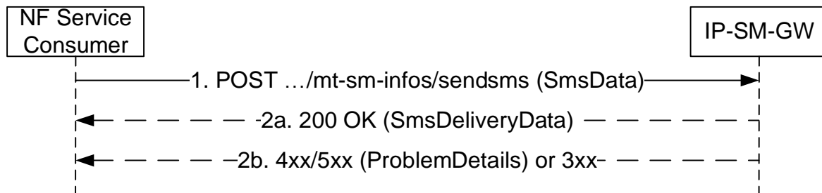
Figure 5.2.2.3.1-1: Transmit downlink SMS message
