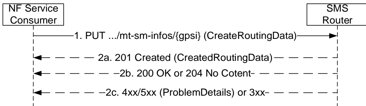
Figure 5.3.2.2.1-1: Routing Information creation
