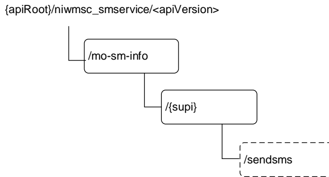
Figure 6.1.3.1-1: Resource URI structure of the Niwmsc_SMSservice API
