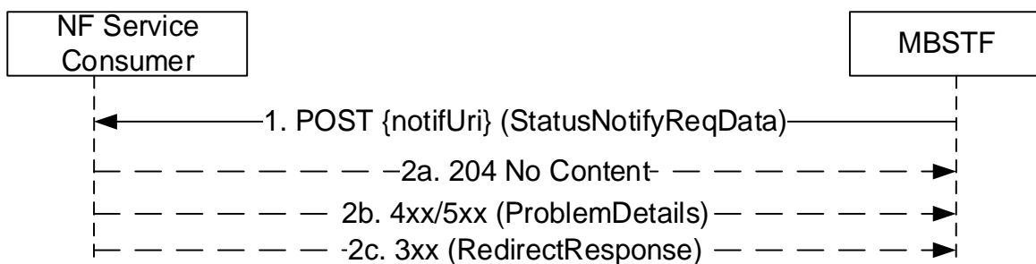
Figure 5.2.2.8.1-1: MBTSMF notifications
