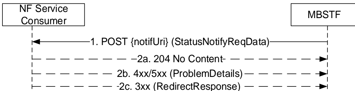
Figure 5.2.2.8.1-1: MBTSMF notifications
