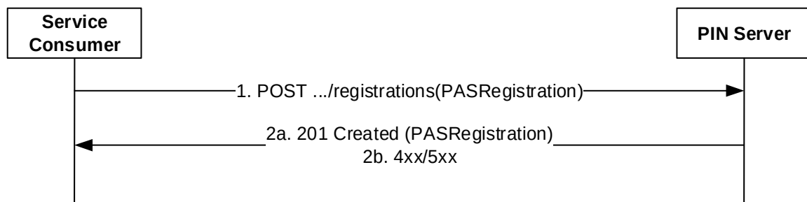
Figure 5.2.2.2-1: Procedure for PAS Registration Creation
