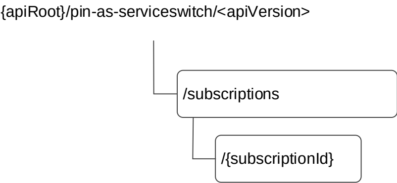
Figure 6.2.3.1-1: Resource URI structure of the PIN_ASServiceSwitch API
