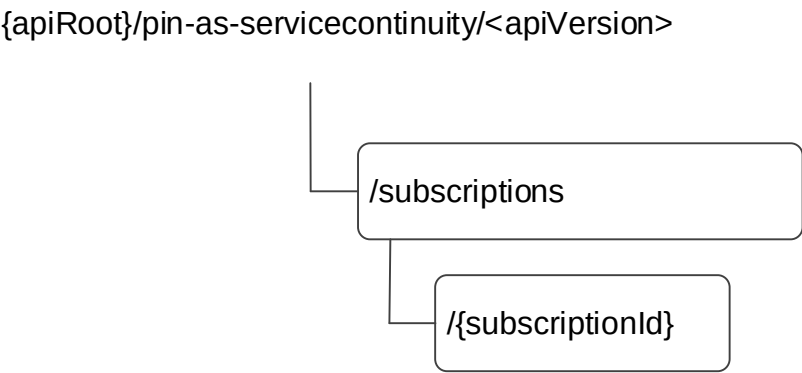
Figure 6.3.3.1-1: Resource URI structure of the PIN_ASServiceContinuity API
