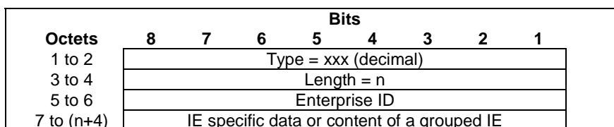
Figure 8.1-3: Vendor-Specific Information Element Format
