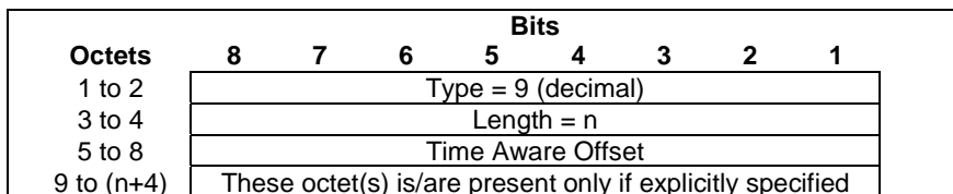
Figure 8.2.13-1: Time Aware Offset
