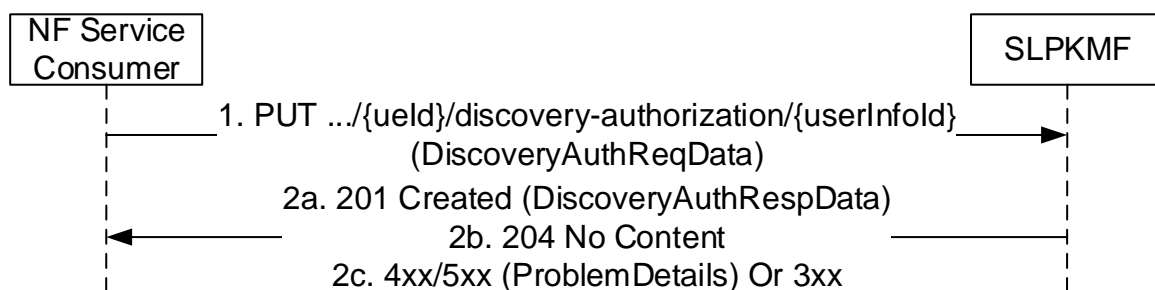
Figure 5.2.2.4.1-1: Discover Authorization
