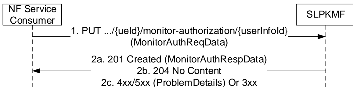
Figure 5.2.2.3.2-1: Monitor Authorization
