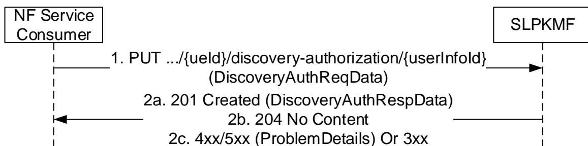
Figure 5.2.2.4.1-1: Discover Authorization
