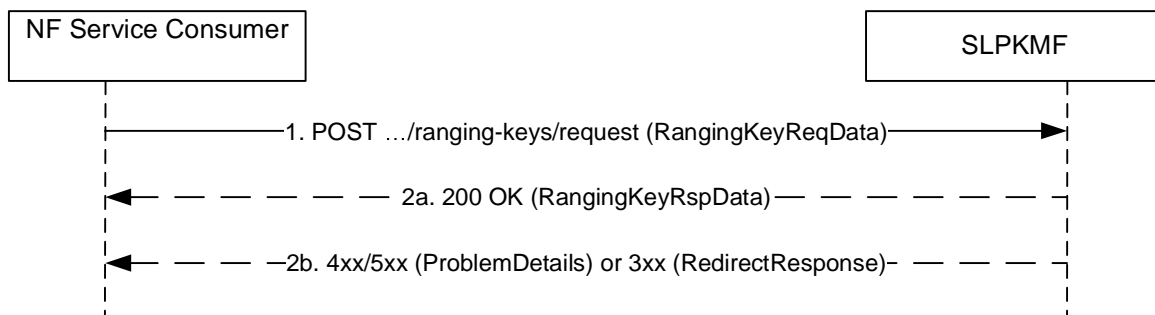
Figure 5.3.2.2.1-1 UnicastKey service operation
