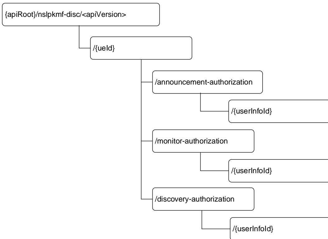
Figure 6.1.3.1-1: Resource URI structure of the Nslpkmf_Discovery API
