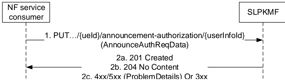
Figure 5.2.2.2.1-1: Announcement Authorization
