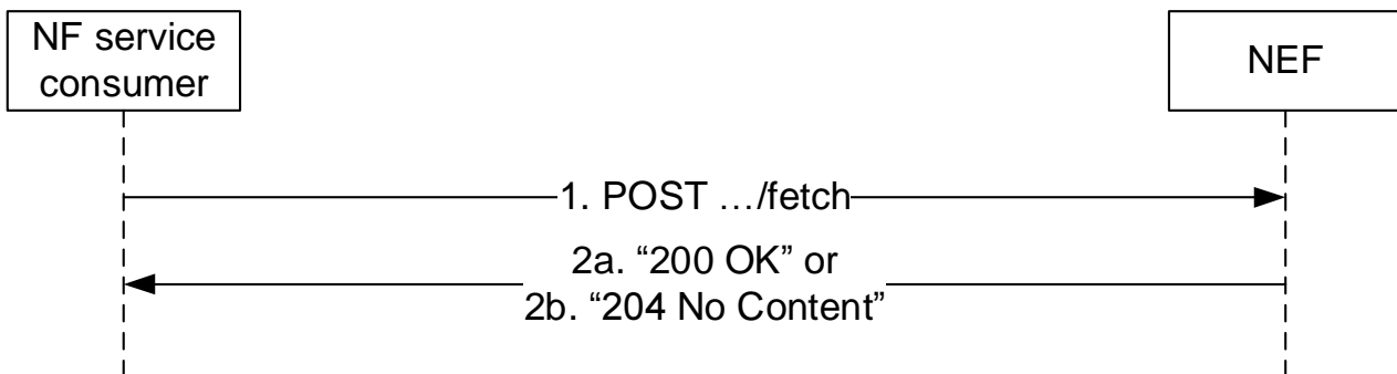
Figure 4.7.2.2.2-1: Fetch internal UE ID for roaming UE
