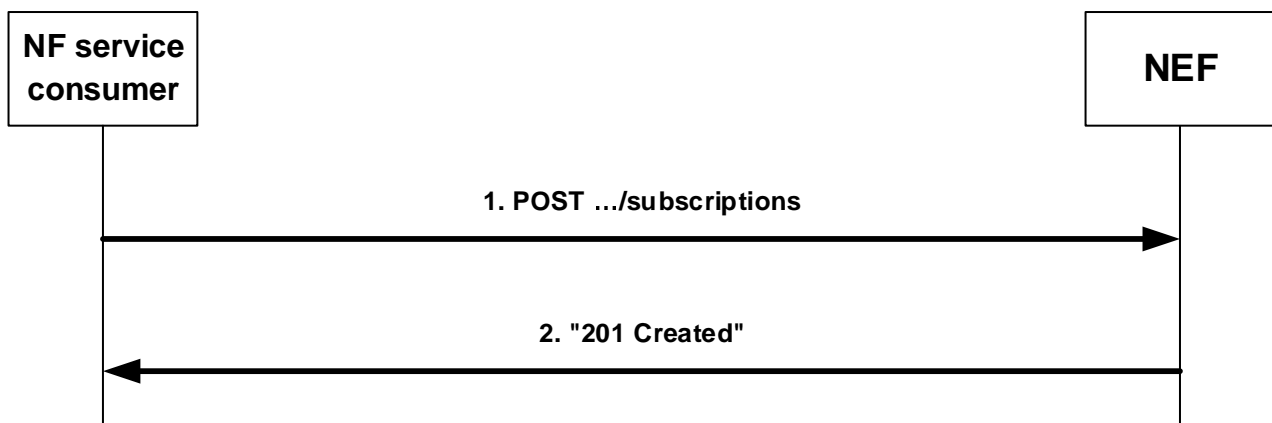
Figure 4.6.2.2-1: Creation of a subscription
