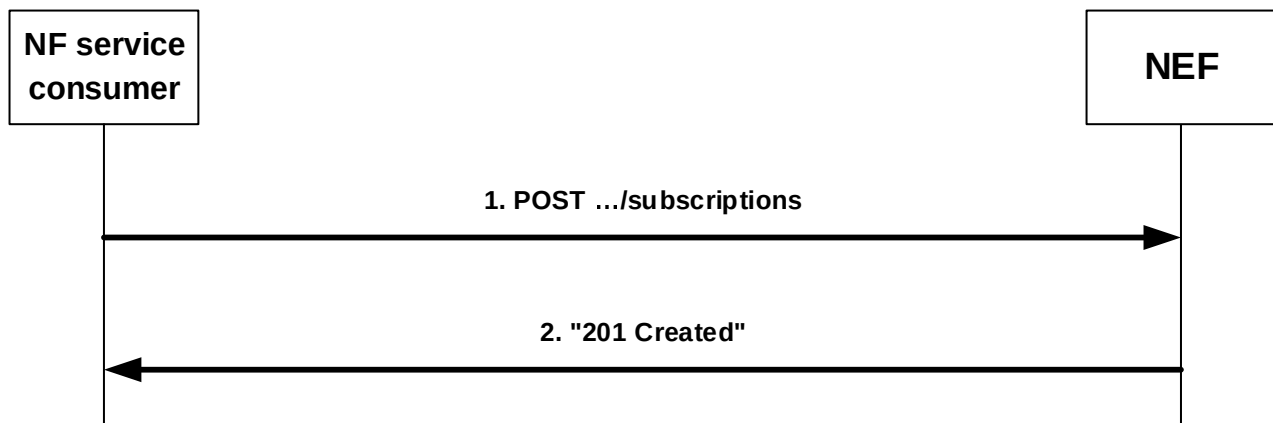
Figure 4.5.2.2.2-1: Creation of a subscription
