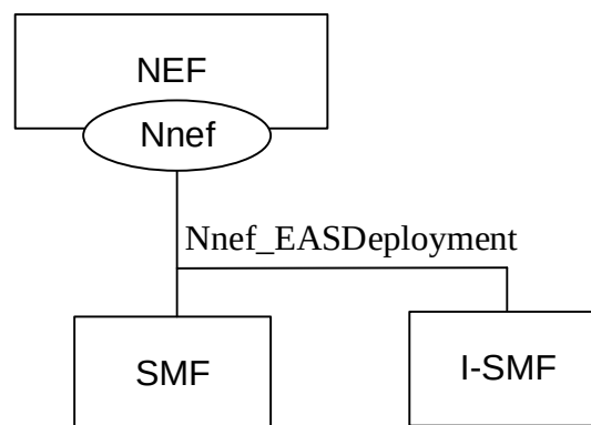
Figure 4.3.1.2-1: Reference Architecture for the Nnef_EASDeployment Service; SBI representation
