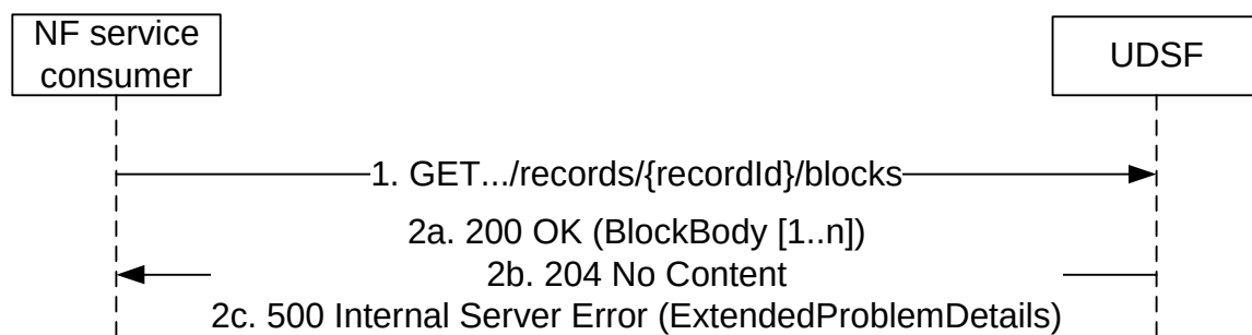
Figure 5.2.2.2.4-1: Requesting Blocks
