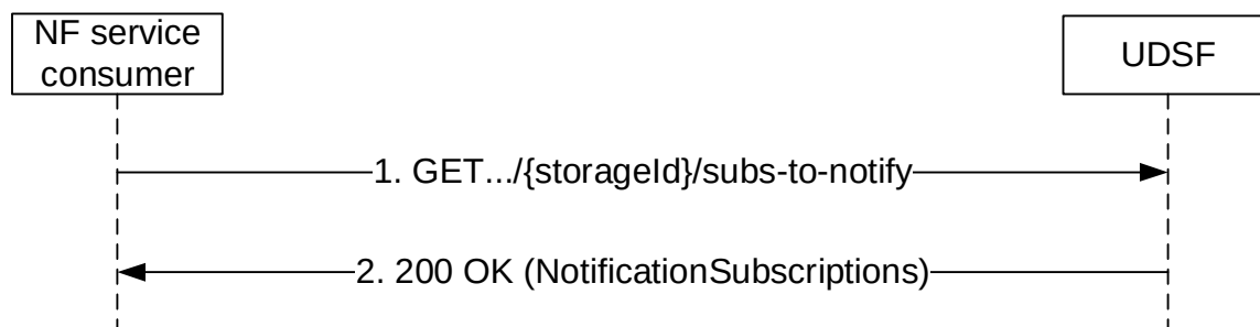
Figure 5.2.2.2.7-1: Requesting Subscriptions
