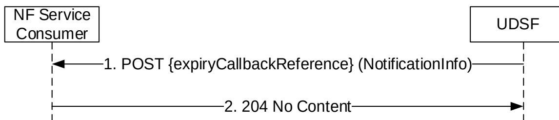
Figure 5.2.2.6.4-1: Subscription Expiry Notification
