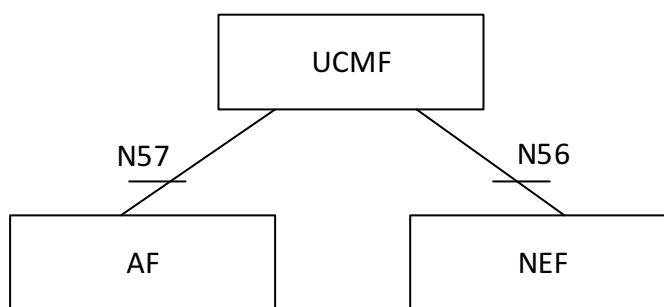
Figure 4.1.2-2: Nucmf_Provisioning service Architecture, reference point representation
