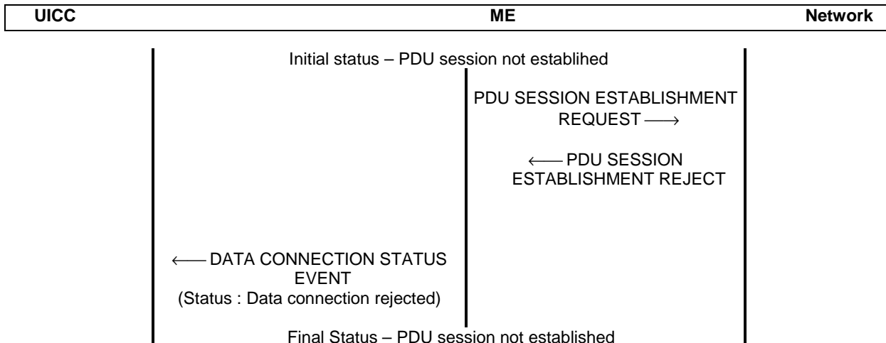
Figure T.3.2 Rejected PDU context activation procedure when initiated by the ME
