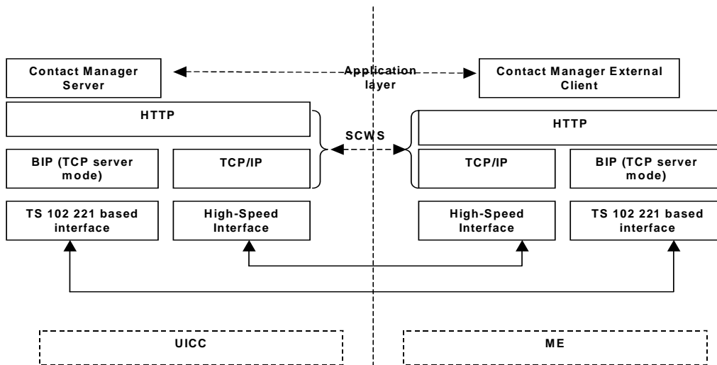
Figure 1: External interface reference model
