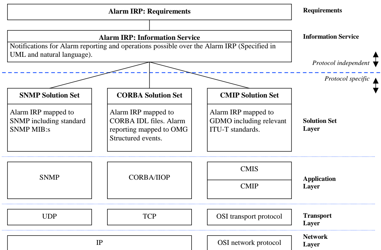
Figure 4.4: Example of an IRP (Alarm IRP)
