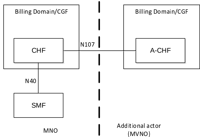
Figure 4.2.6c: 5G data connectivity converged charging architecture in additional actor (i.e. MVNO owning a CHF, referred to as A-CHF) scenario in reference point representation
