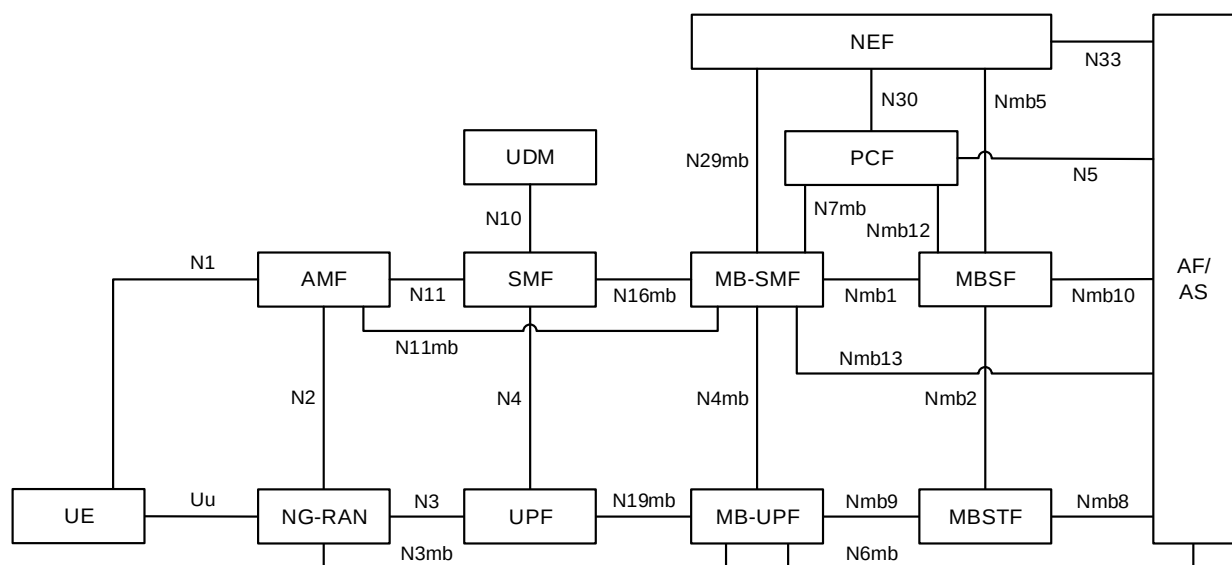
Figure 4.1.9.1: Non-roaming architecture for 5G Multicast and Broadcast Service in reference point representation
