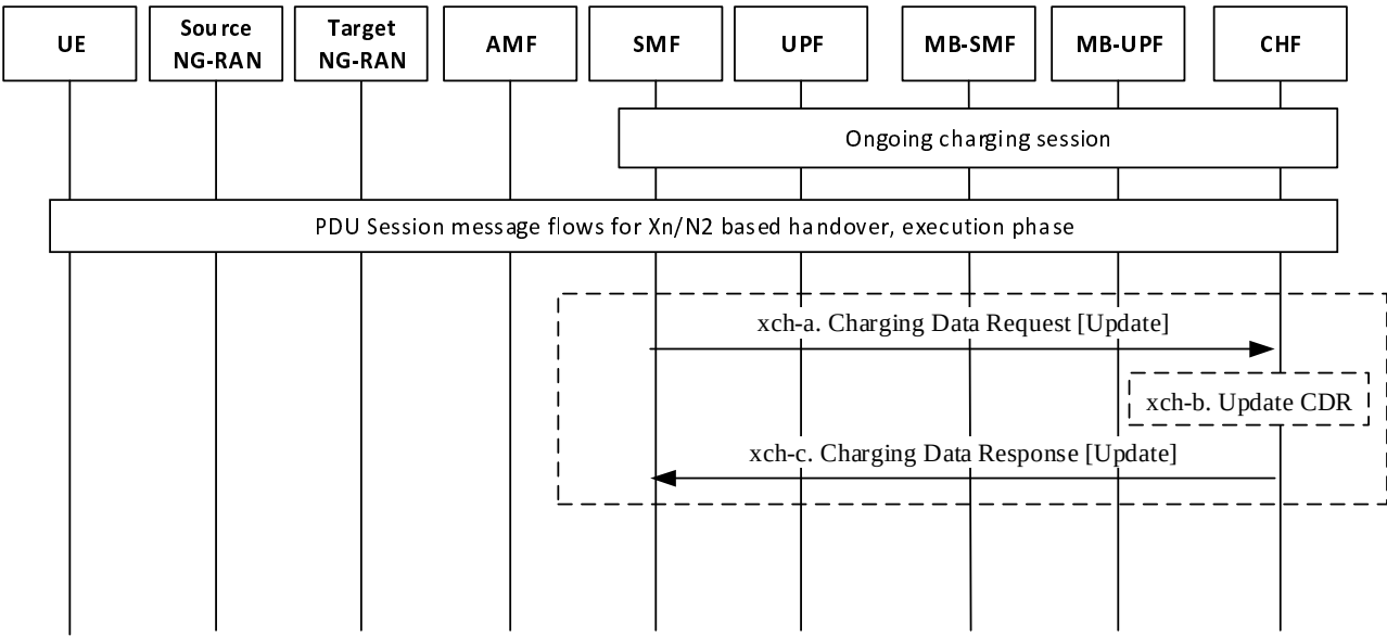
Figure 5.2.24.3.1: Xn/N2 based handover, execution phase
