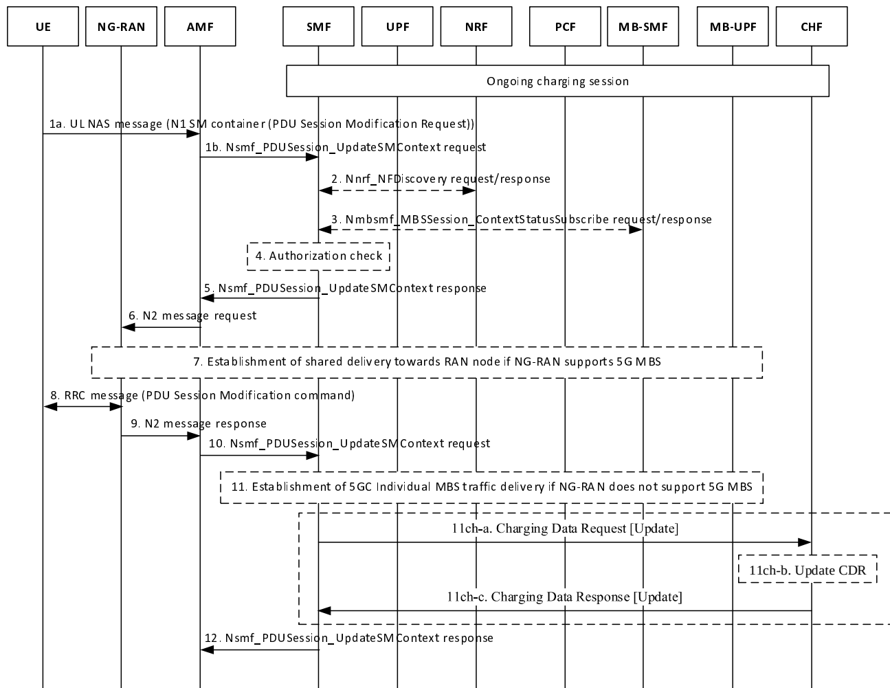
Figure 5.2.2.24.2.1: UE initiated multicast session join
