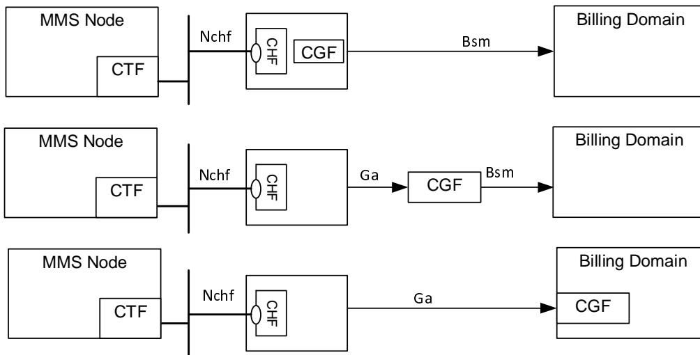
Figure 4.4.1: MMS converged charging architecture
