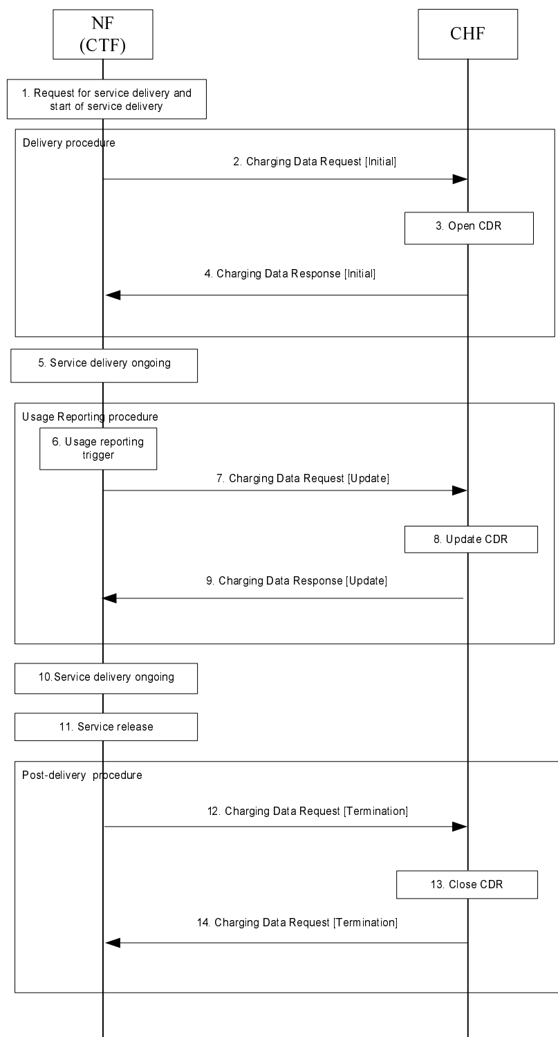
Figure 5.1.2.2.1: Offline charging
