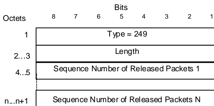
Figure 6.2.4.5.4.1: Sequence Numbers of Released Packets IE
