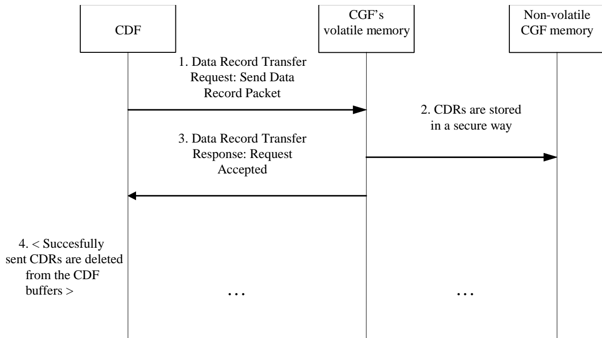
Figure 5.2.2.1.1: Normal CDR transfer process between a CDF and CGF
