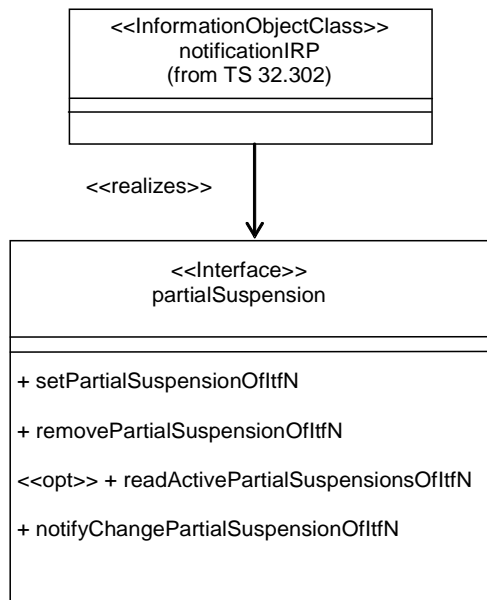
Figure 6.1-1: Class Diagram for AlarmIRPOperation_6 Interface
