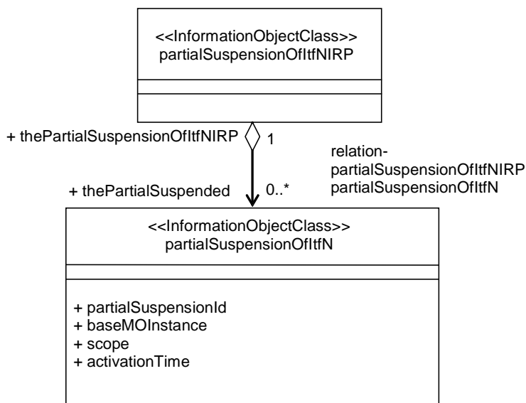
Figure 5.2.1-1: Class Diagram
