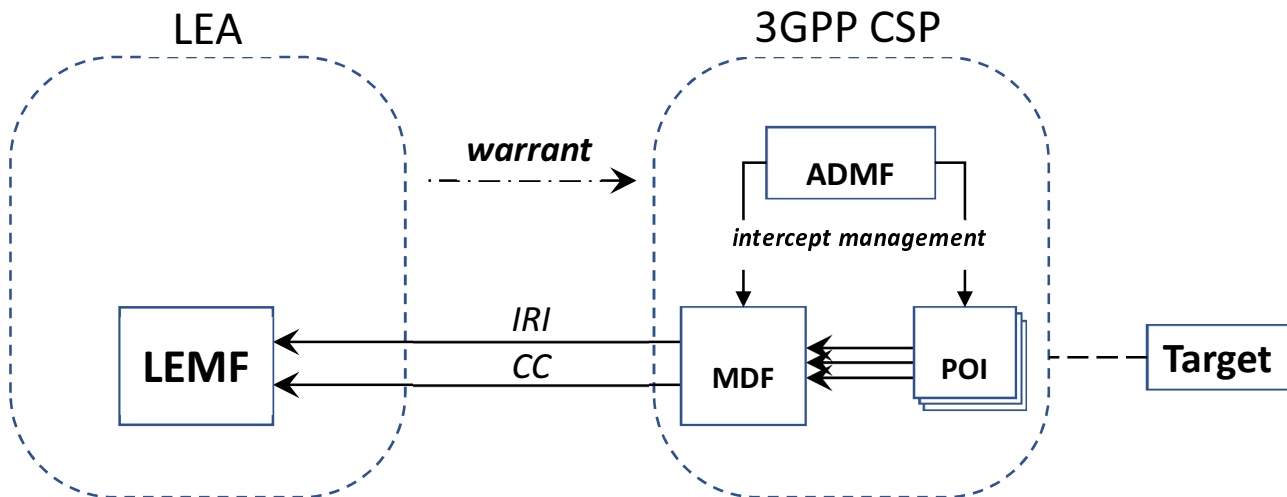
Figure 5.2-1: Generic Lawful Interception model
