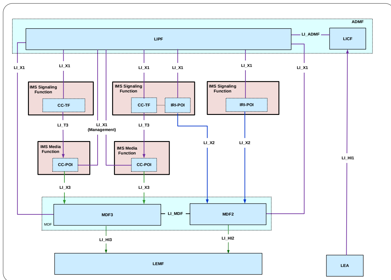
Figure 7.4.2.1-1: IMS LI architecture
