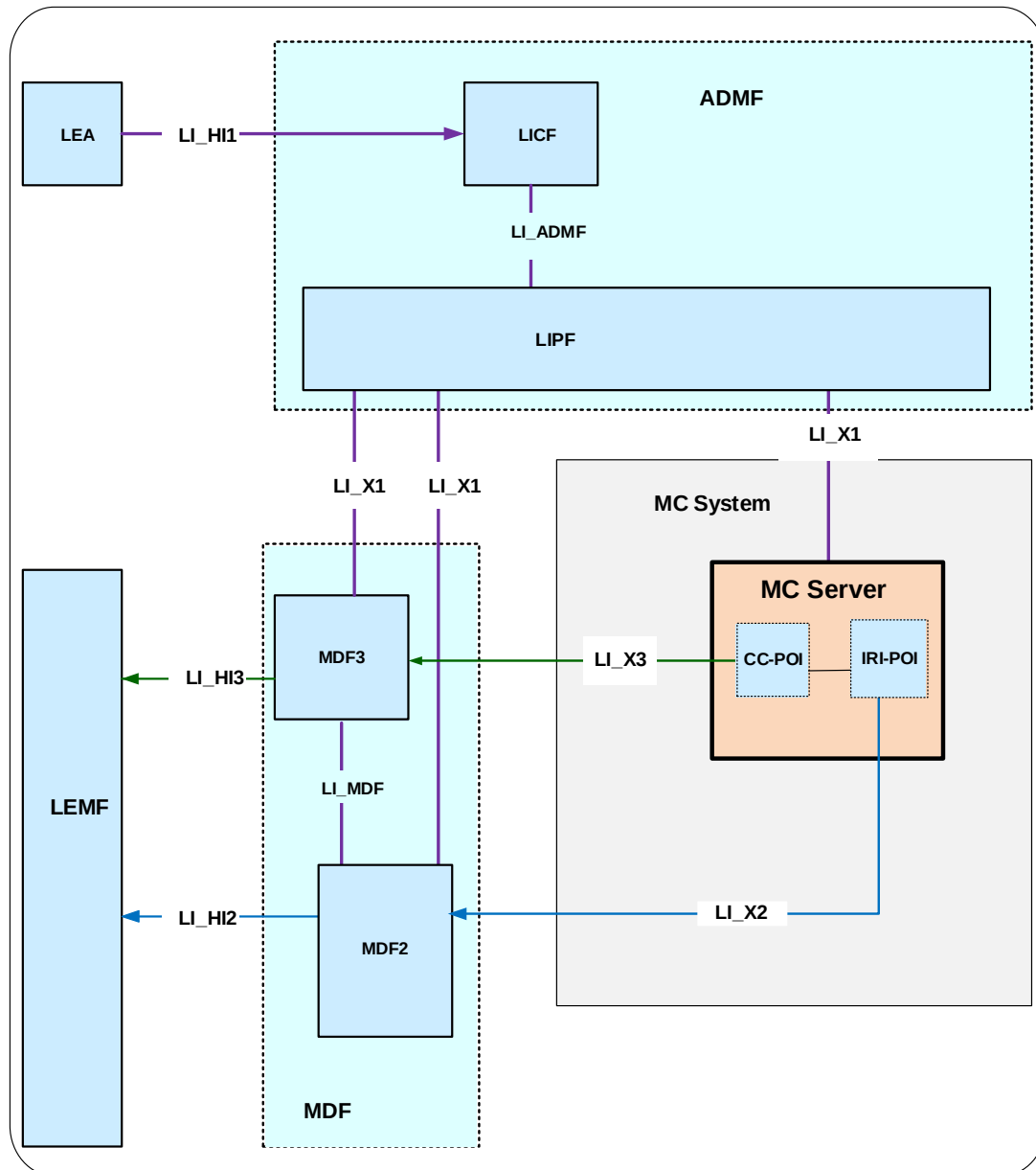
Figure 7.23.2-1: LI architecture for Mission Critical Services
