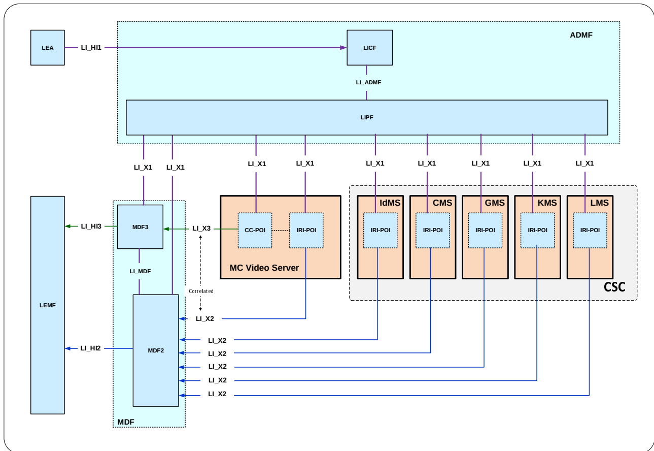
Figure 7.23.4.2-1: LI architecture for MCVideo
