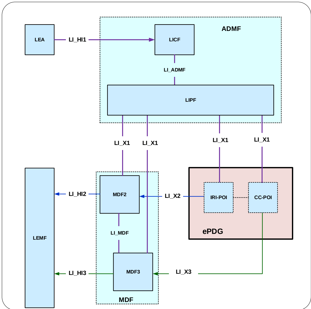
Figure 6.3.4.1-1: LI architecture for LI at ePDG
