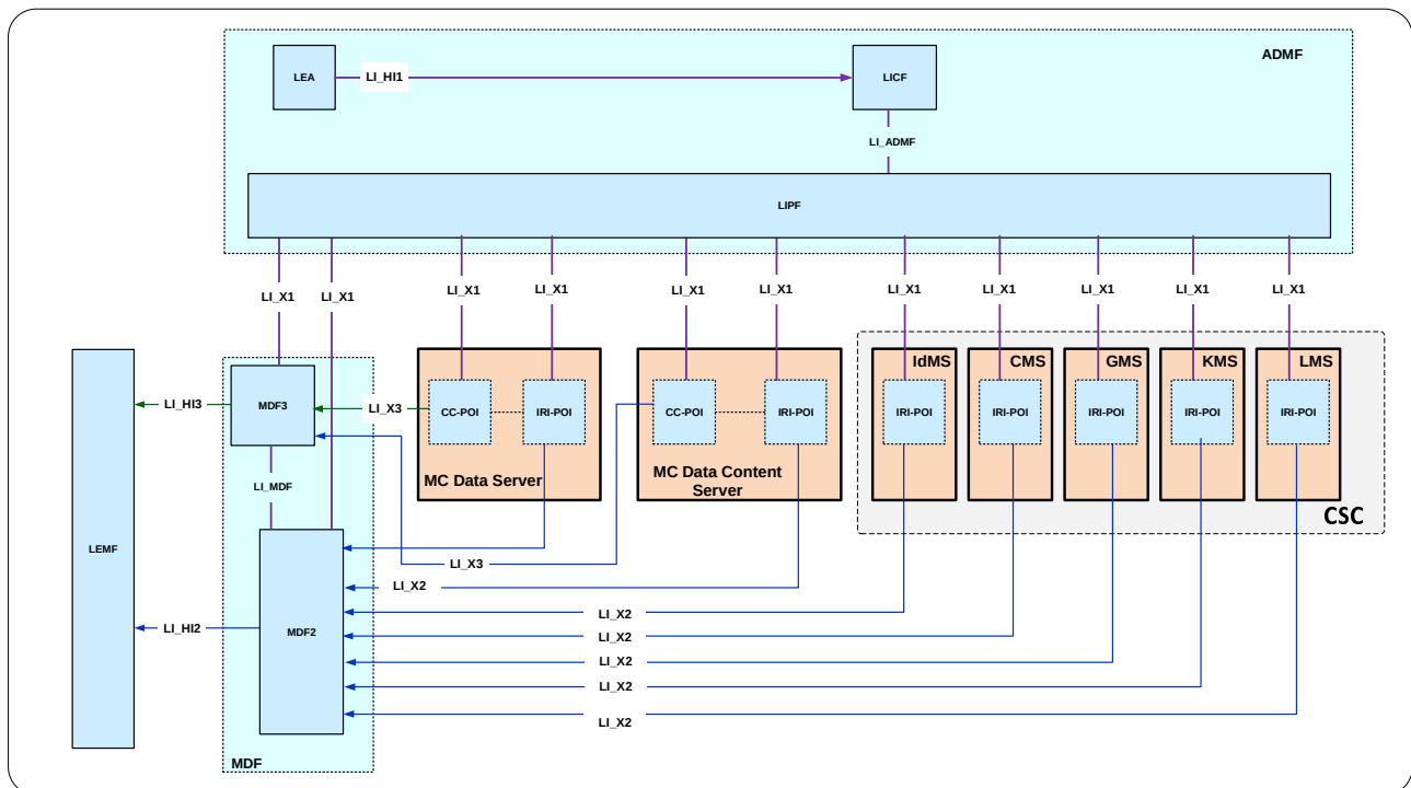
Figure 7.23.5.2-1: LI architecture for MCDData
