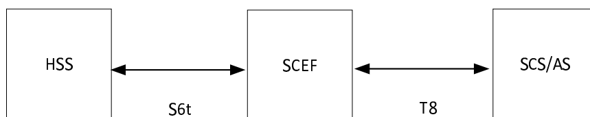
Figure 7.11.5.1-1: EPS architecture for Parameter Provisioning
