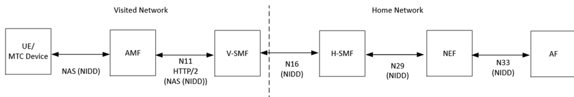
Figure 7.8.1.3.1-1: 5GS Architecture for NIDD using NEF in roaming situation
