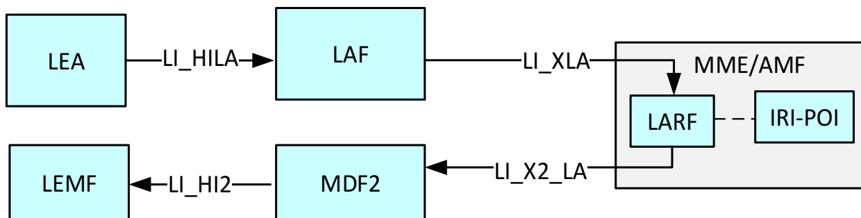
Figure 7.3.5.2.2-1: Delivery of the retrieved information via the LI_HI2
