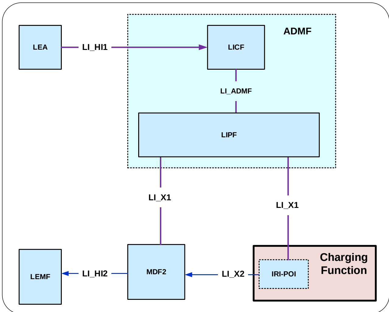
Figure 7.22.1-1: Architecture for LI at the Charging Function
