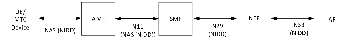
Figure 7.8.1.2.1-1: 5GS Architecture for NIDD using NEF
