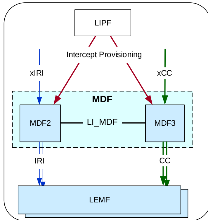
Figure 5.3.4-1: MDF2 and MDF3
