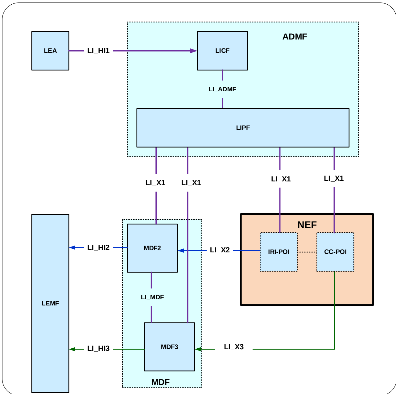
Figure 7.9.2.1-1: LI architecture for NIDD using NEF showing LI at NEF
