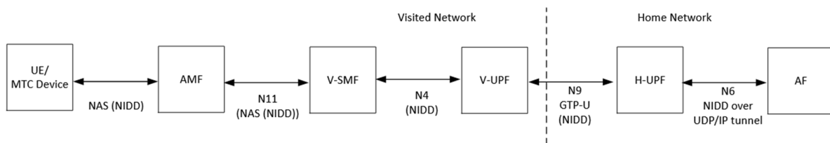
Figure 7.8.1.3.2-1: 5GS Architecture of NIDD using a PtP N6 tunnel in roaming situation
