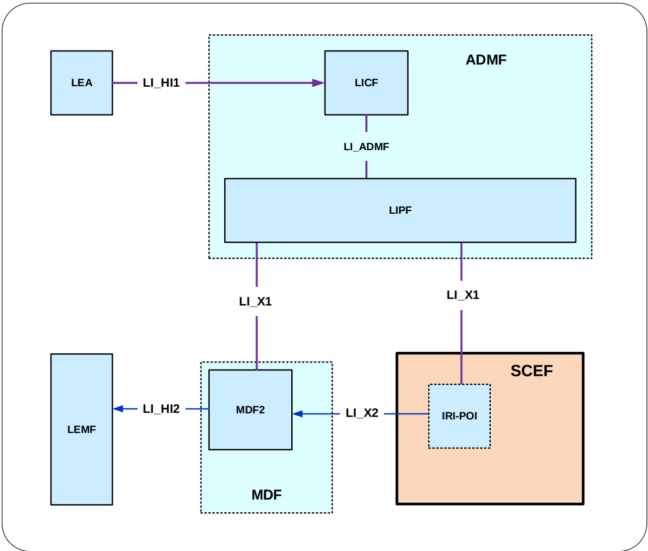
Figure 7.11.3.2-1: LI architecture for device triggering using SCEF
