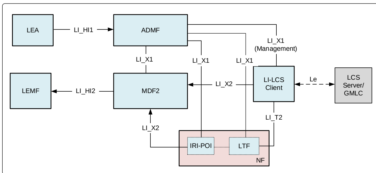
Figure 7.3.3.3-1: LALS model for triggered location (POI/LTF option)
