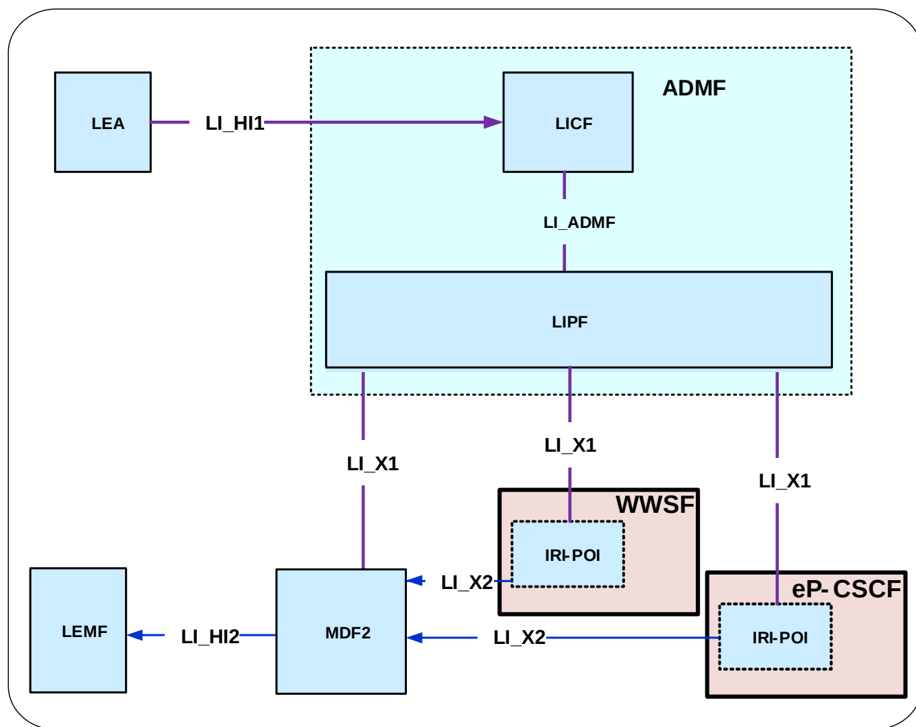
Figure 7.19.2-1 LI architecture for WebRTC access to the IMS
