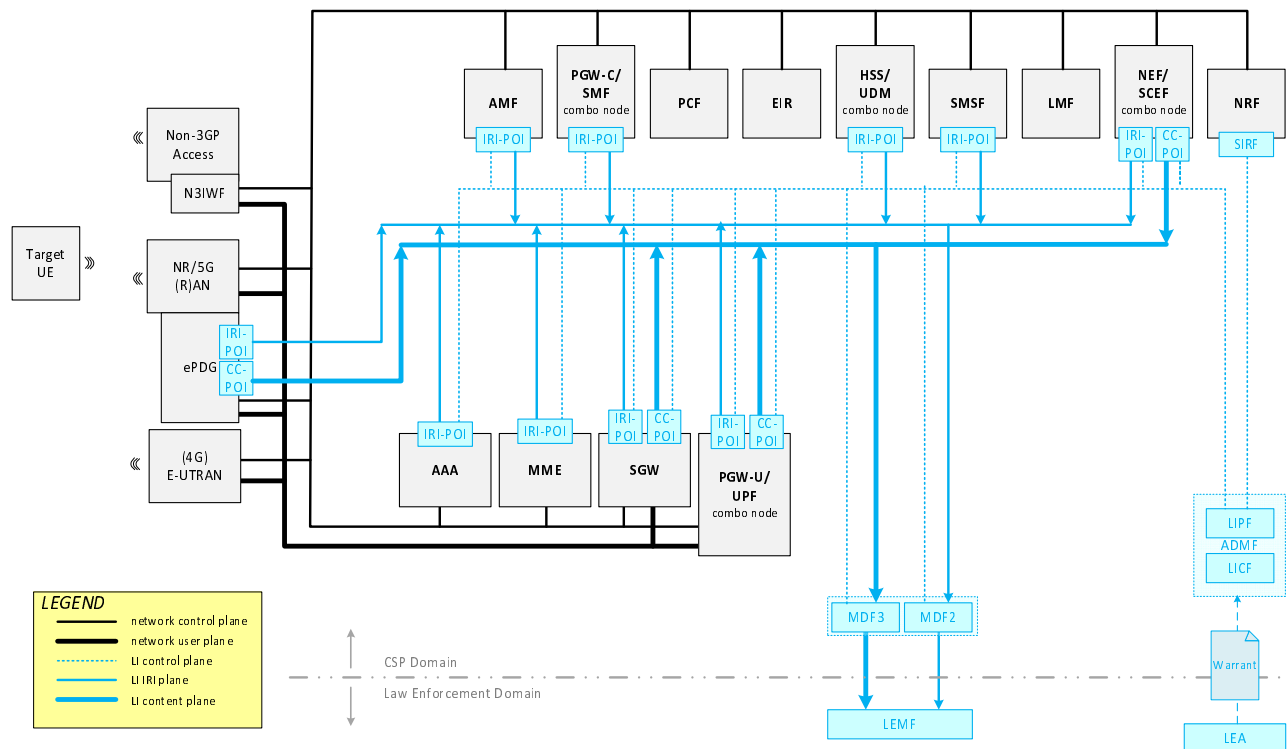
Figure 6.6-1: EPC/5G Interworking LI architecture
