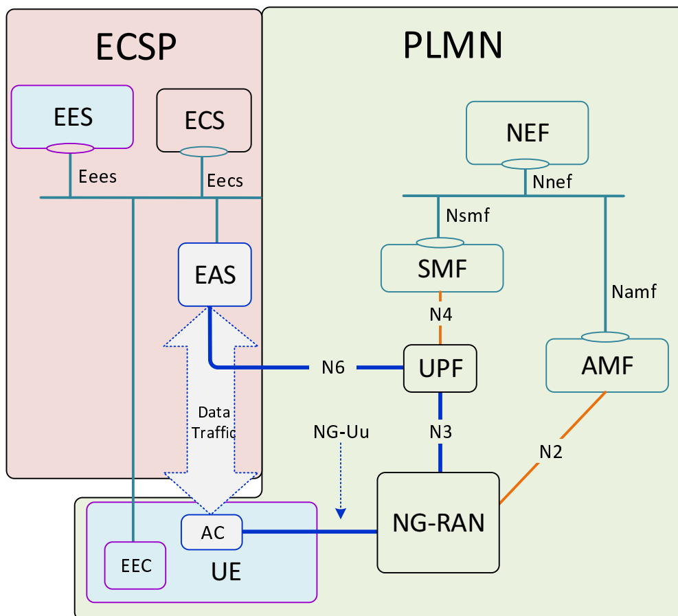
Figure 7.16.1-1: Edge computing network
