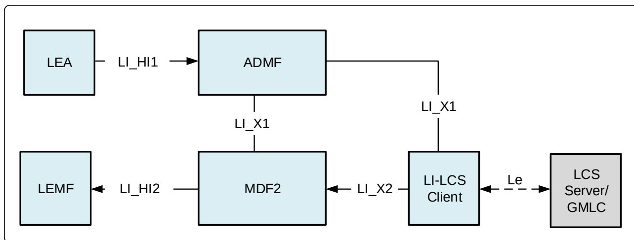
Figure 7.3.3.2.1-1: LALS model for target positioning
