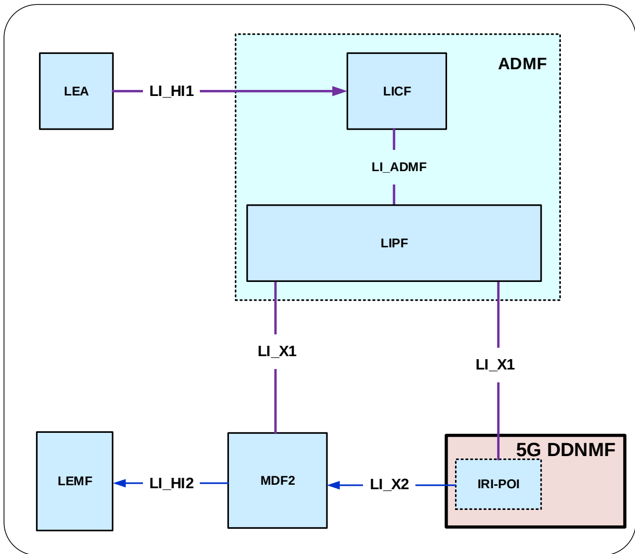
Figure 7.20.2-1: LI architecture for 5G ProSe showing LI at 5G DDNMF
