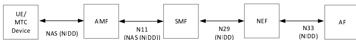
Figure 7.8.1.2.1-1: 5GS Architecture for NIDD using NEF
