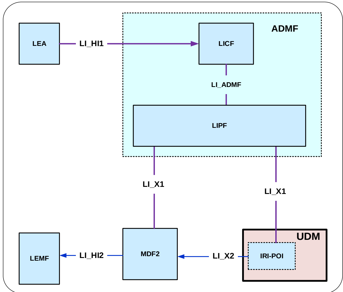
Figure 7.2.2.1-1: LI architecture for LI at UDM
