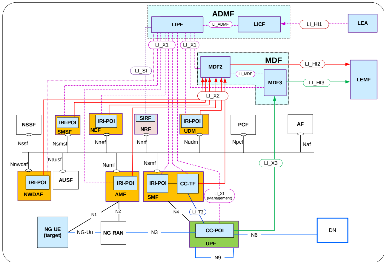
Figure A.1.2-1: Network topology showing LI for 5G (service-based representation) with point-to-point LI system
