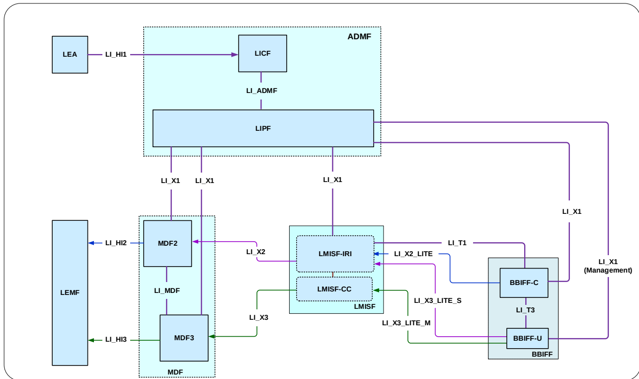
Figure 7.4.7.4.2-1: VPLMN generic LI architecture for home-routed roaming
