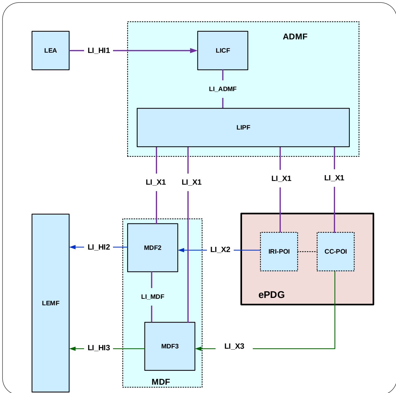
Figure 6.3.4.1-1: LI architecture for LI at ePDG
