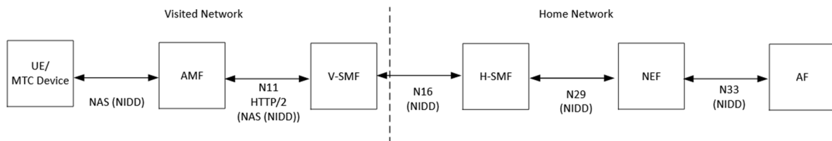
Figure 7.8.1.3.1-1: 5GS Architecture for NIDD using NEF in roaming situation
