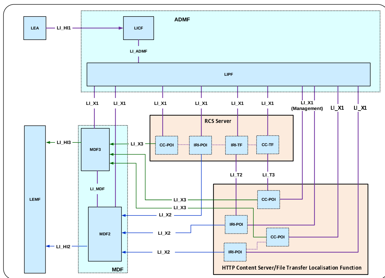
Figure 7.13.2.1-1: LI architecture for RCS services
