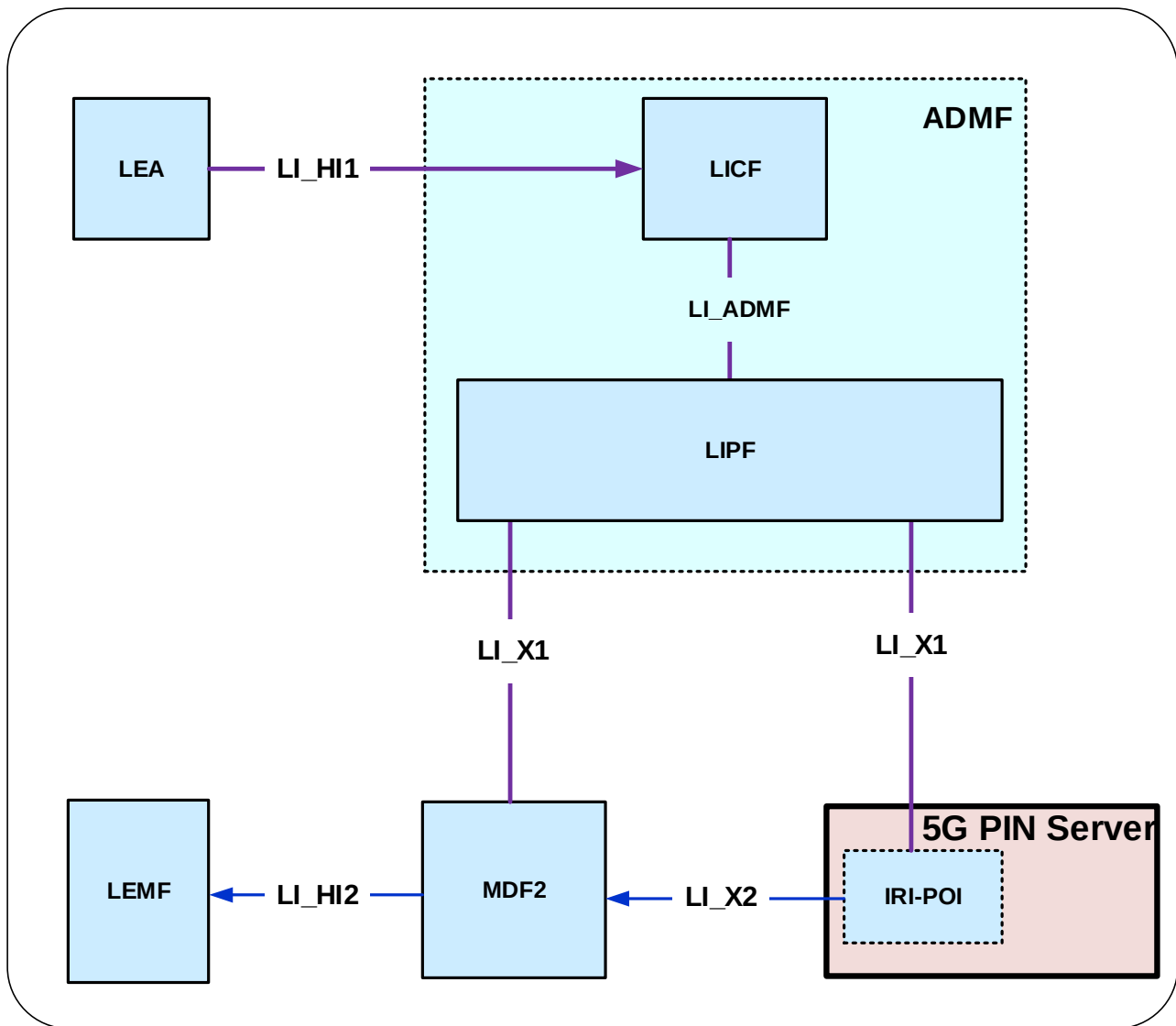
Figure 7.21.2-1: LI architecture for Personal IoT showing LI at 5G PIN Server
