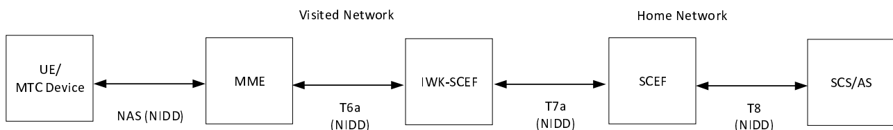
Figure 7.10.1.3.1-1: EPS Architecture for NIDD using SCEF in roaming situation
