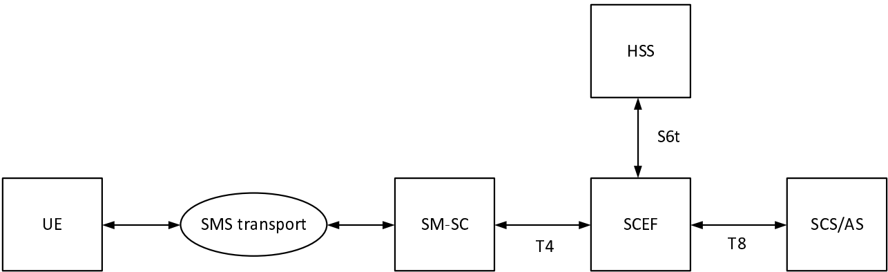
Figure 7.11.3.1-1: EPS architecture for device triggering
