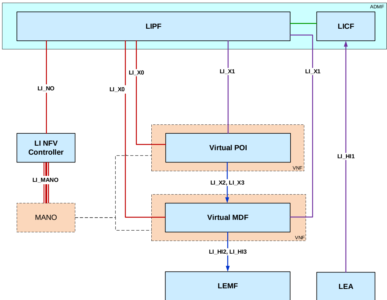
Figure 5.6.2-1: Simplified virtualised LI system with provisioning infrastructure for a direct provisioned POI
