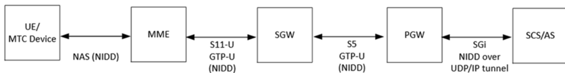
Figure 7.10.1.2.2-1: EPS Architecture for NIDD using a PtP SGi tunnel
