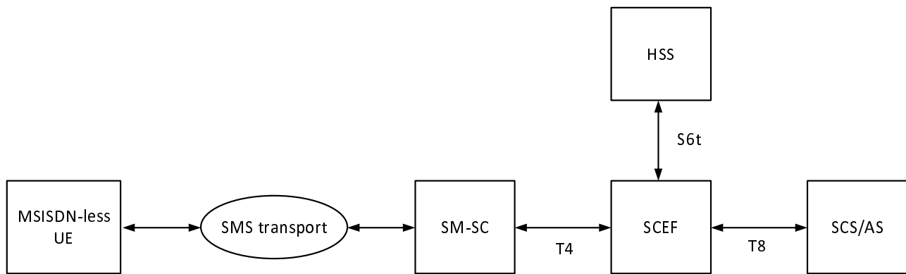
Figure 7.11.4.1-1: EPS architecture for MSISDN-less MO SMS
