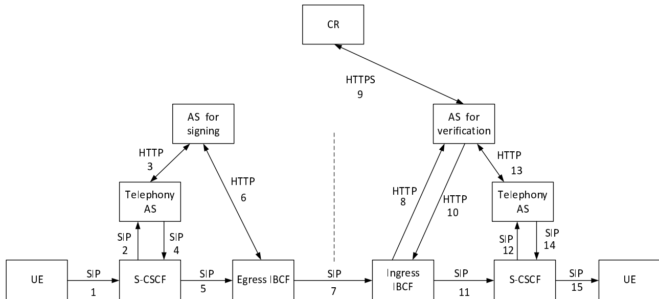
Figure E.4-1: SHAKEN reference call flow using end-to-end SIP signalling
