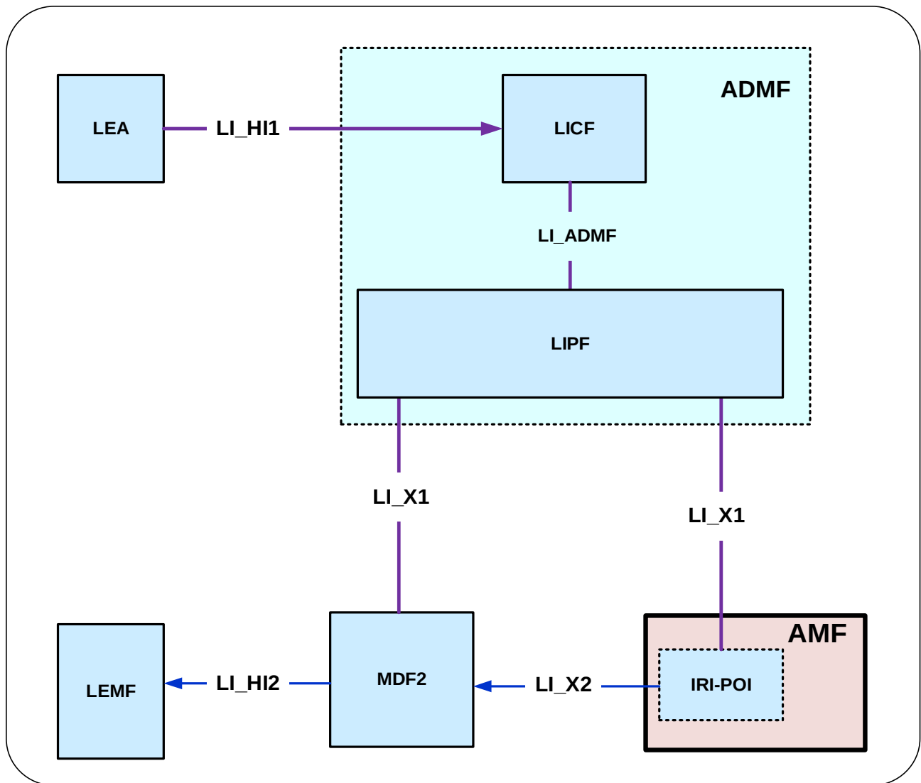
Figure 6.2.2.1-1: LI architecture for LI at AMF
