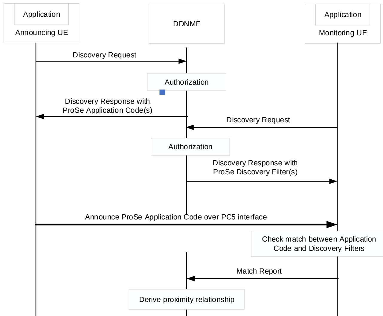
Figure G.2.1-1: High level Direct Discovery procedure
