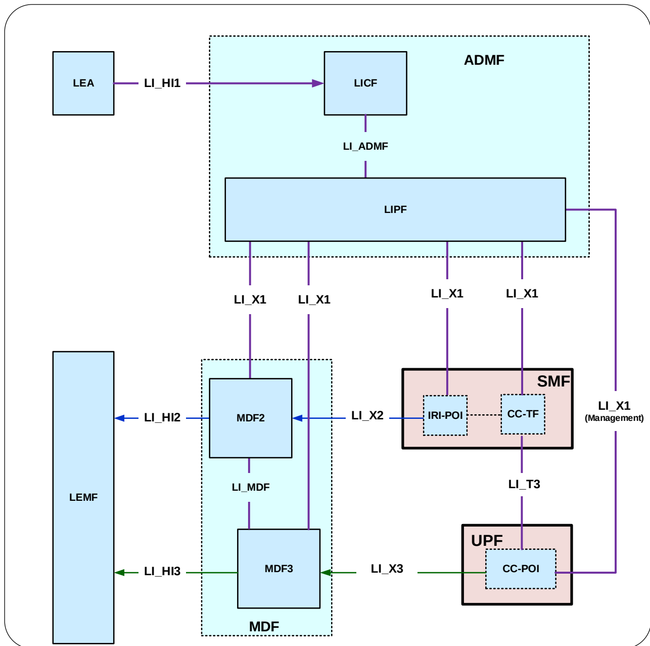
Figure 6.2.3.1-1: LI architecture showing LI at SMF/UPF
