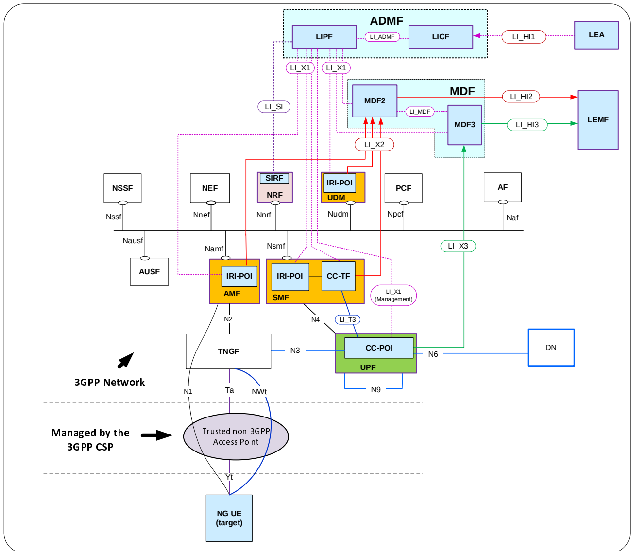
Figure A.4.2-2: Network topology showing LI for non-3GPP access to 5G via TNGF
