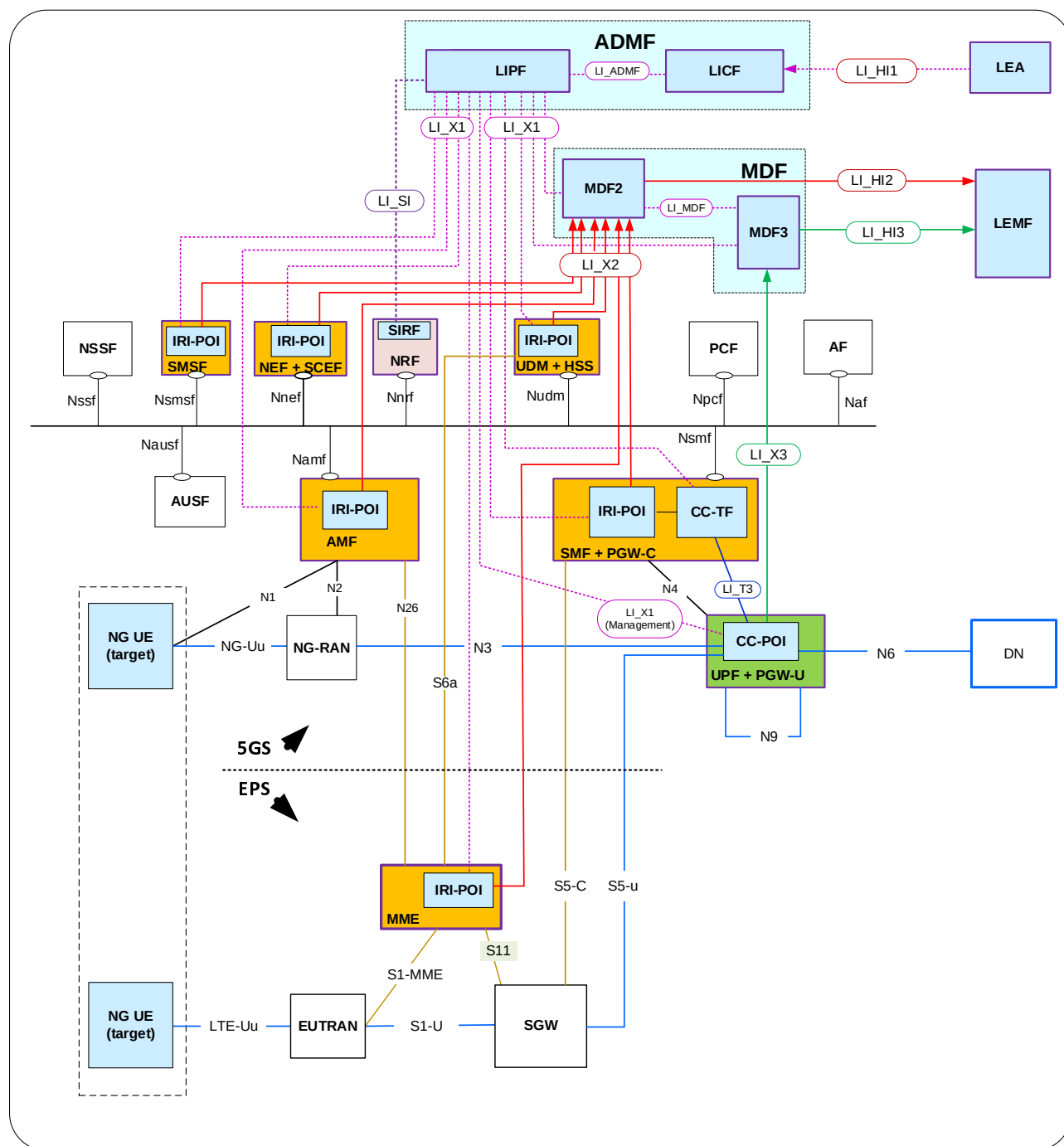
Figure A.2.2-1: Network topology showing LI for interworking with EPC/E-UTRAN
