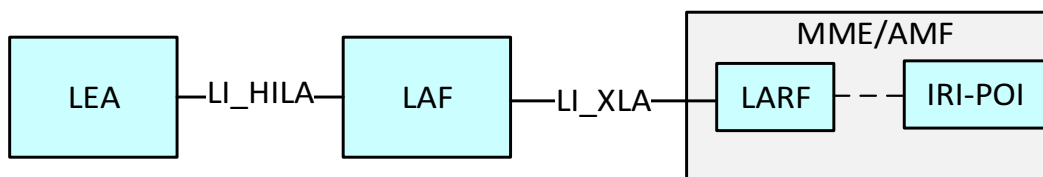
Figure 7.3.5.2.1-1: Delivery of the retrieved information via the LI_HILA
