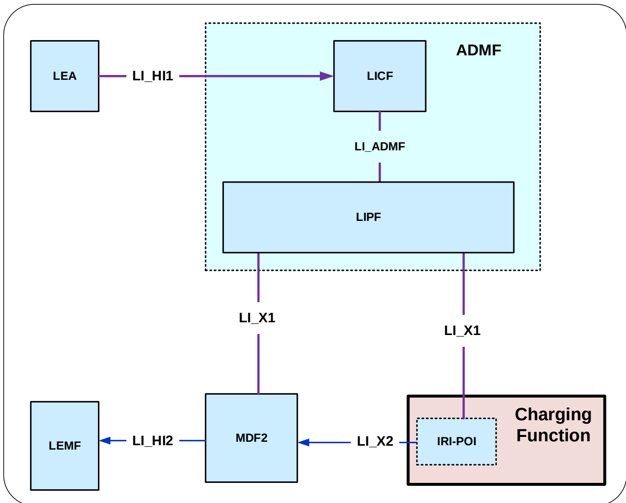
Figure 7.22.1-1: Architecture for LI at the Charging Function
