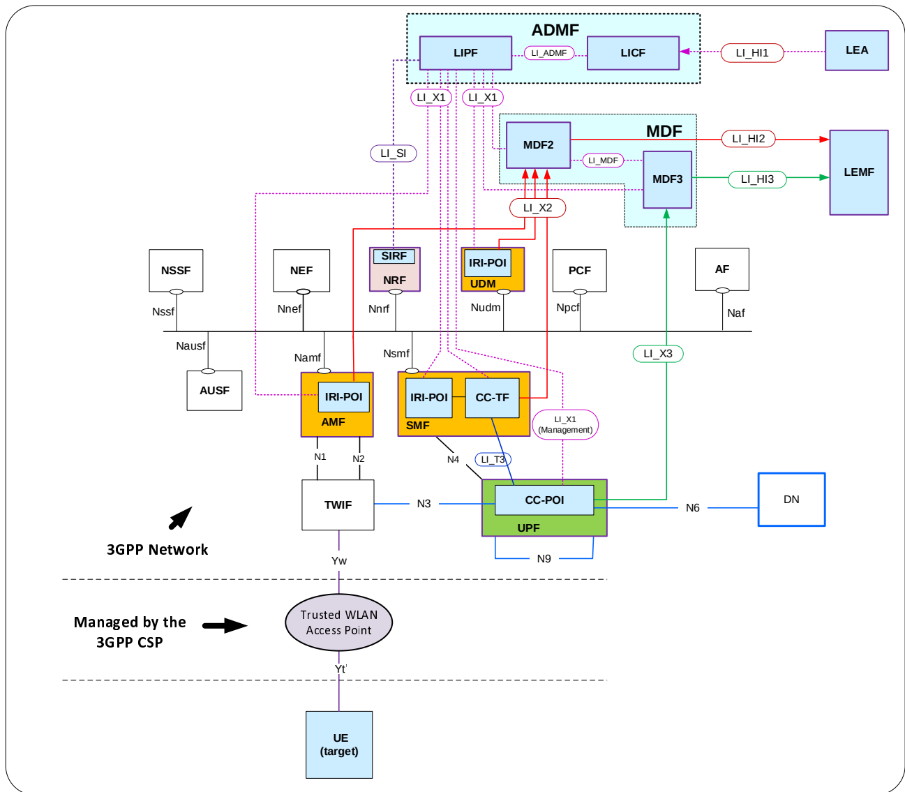
Figure A.4.2-3: Network topology showing LI for non-3GPP access to 5G via TWIF
