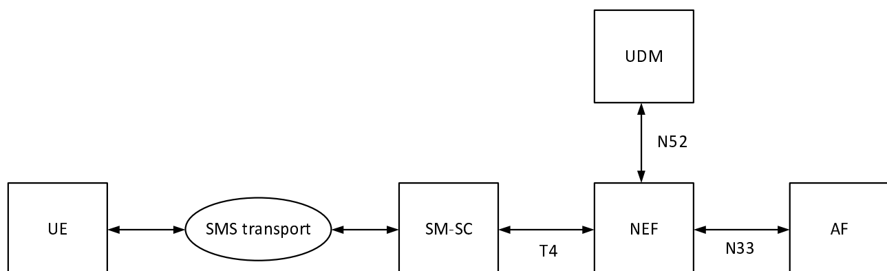
Figure 7.9.3.1-1: 5GS architecture for device triggering
