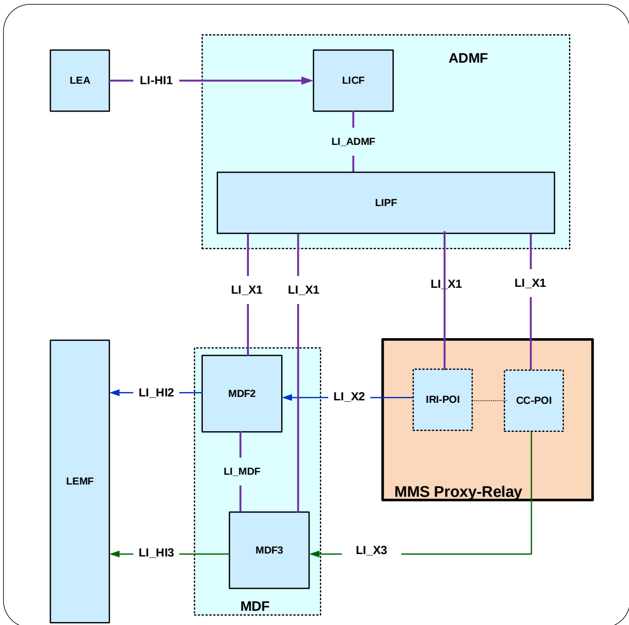
Figure 7.5.2.1-1: LI architecture for MMS showing LI at MMS Proxy-Relay
