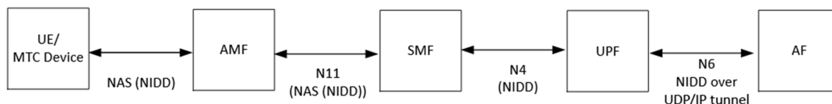
Figure 7.8.1.2.2-1: 5GS Architecture for NIDD using a PtP N6 tunnel
