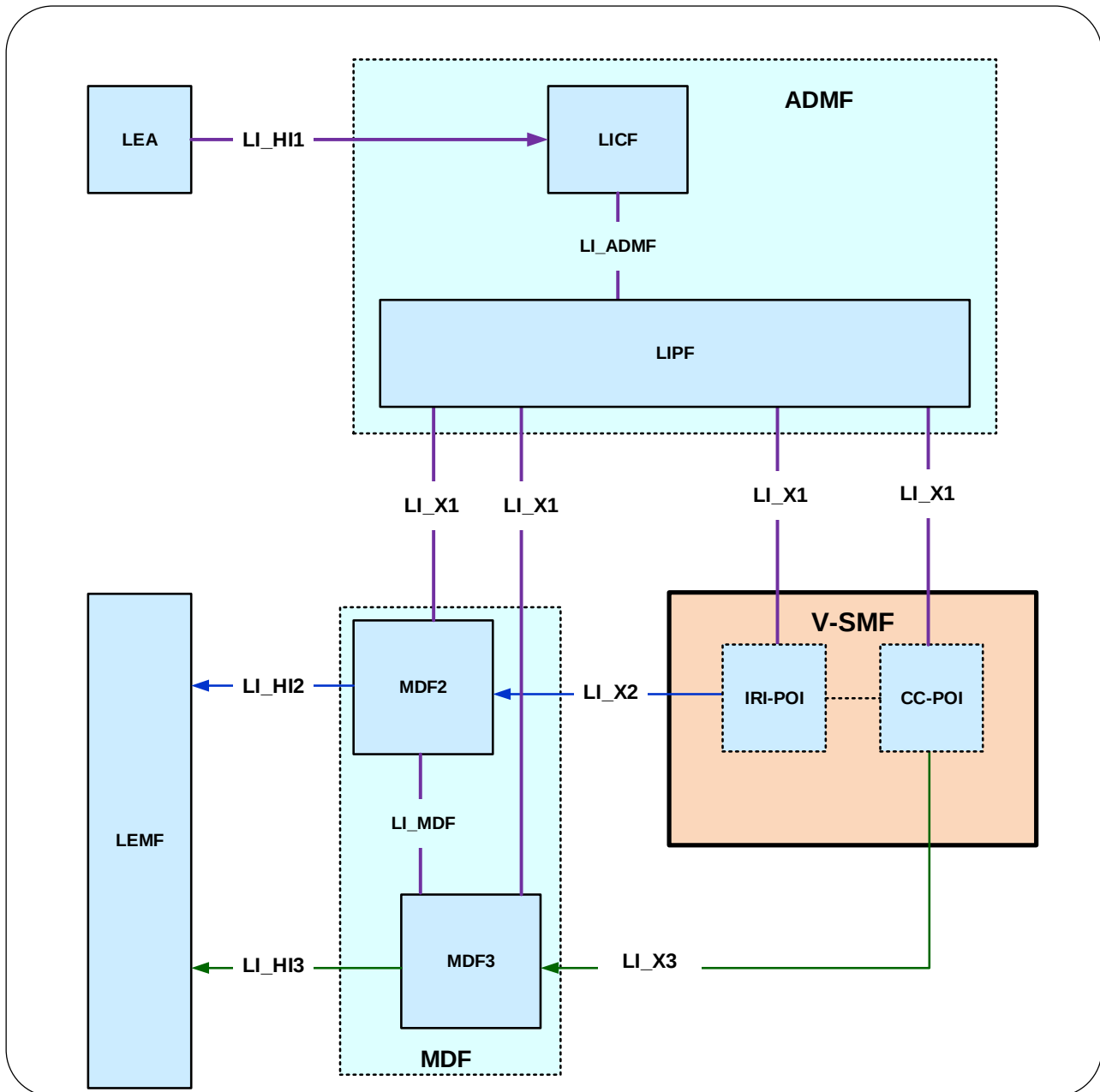
Figure 7.8.2.1.2-1: LI architecture for NIDD using NEF showing LI at V-SMF
