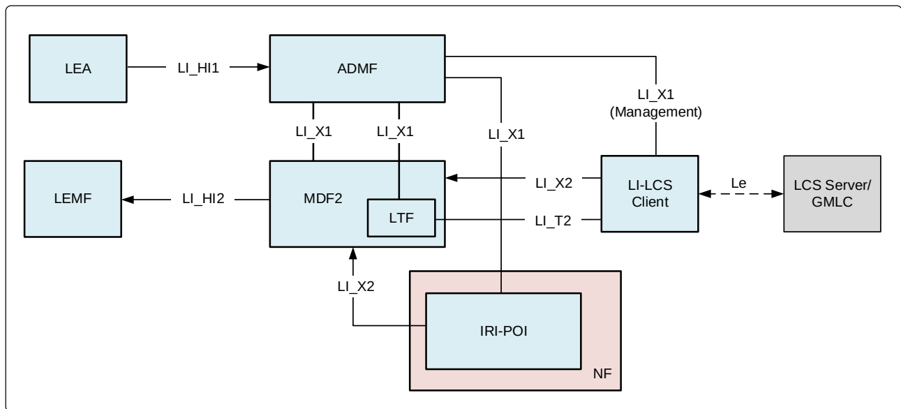
Figure 7.3.3.3-2: LALS Model for triggered location (MDF/LTF option)
