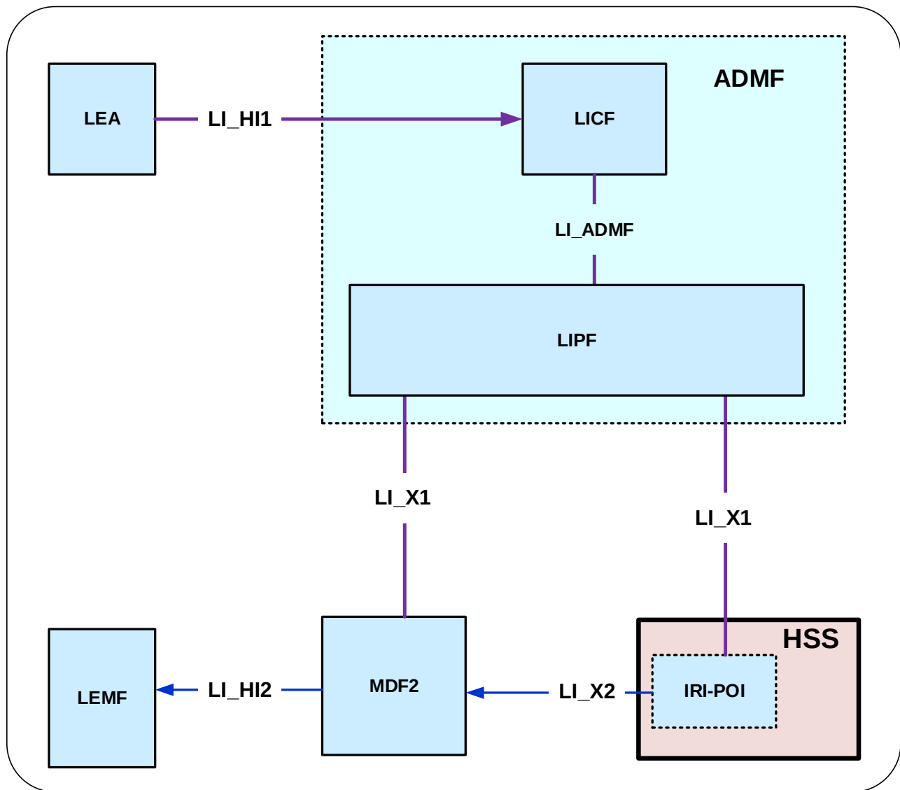
Figure 7.2.3.1-1: LI architecture for LI at HSS
