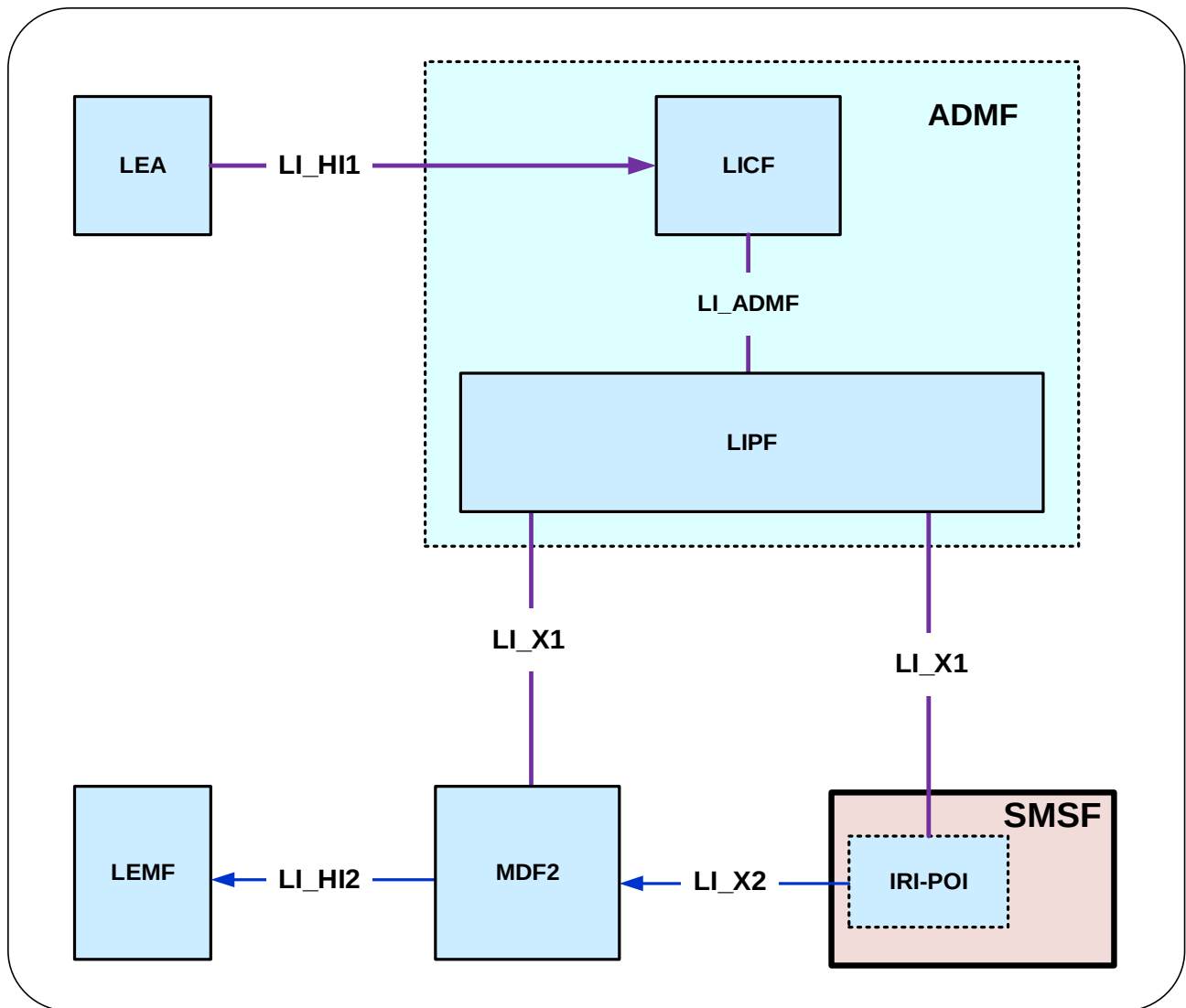
Figure 6.2.5.1-1: LI architecture for LI at SMSF
