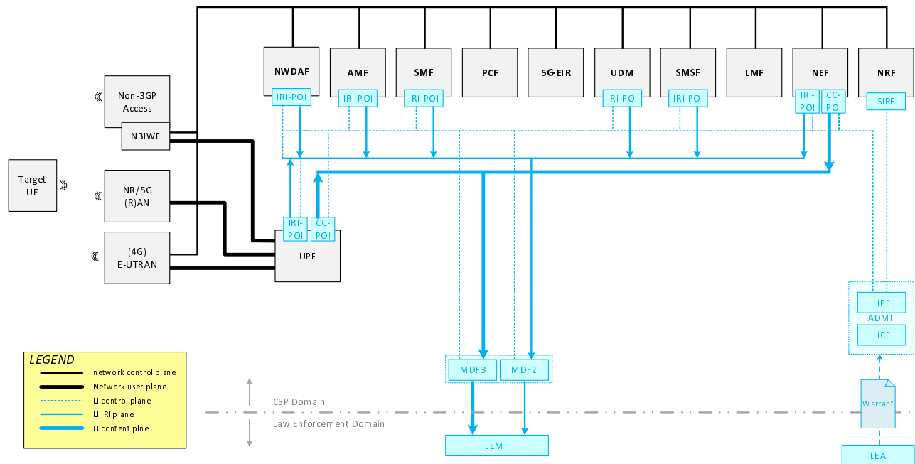
Figure 6.2.1-2: 5G core-anchored LI architecture
