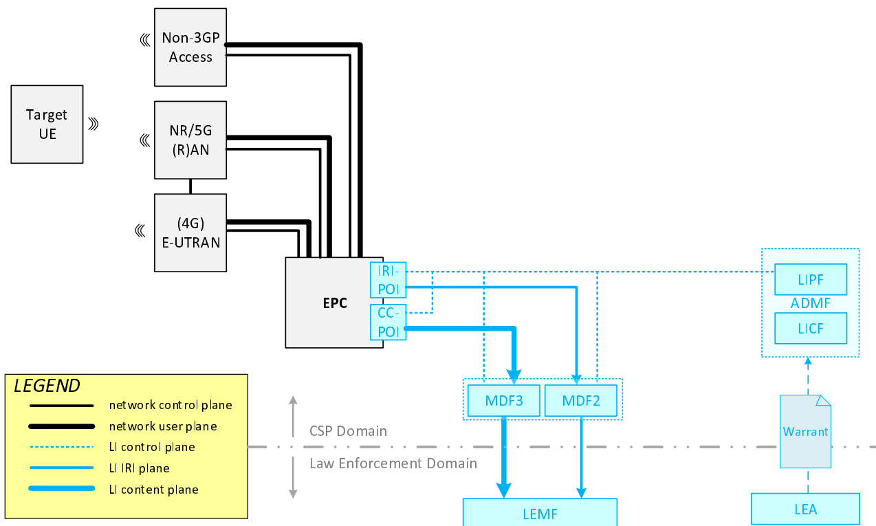
Figure 6.2.1-1: 5G EPC-anchored LI architecture
