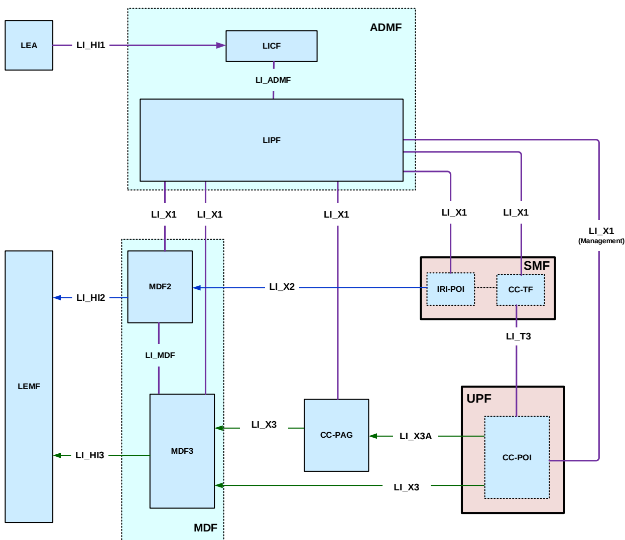
Figure 8.6.2-1: LI architecture showing CC-PAG.
