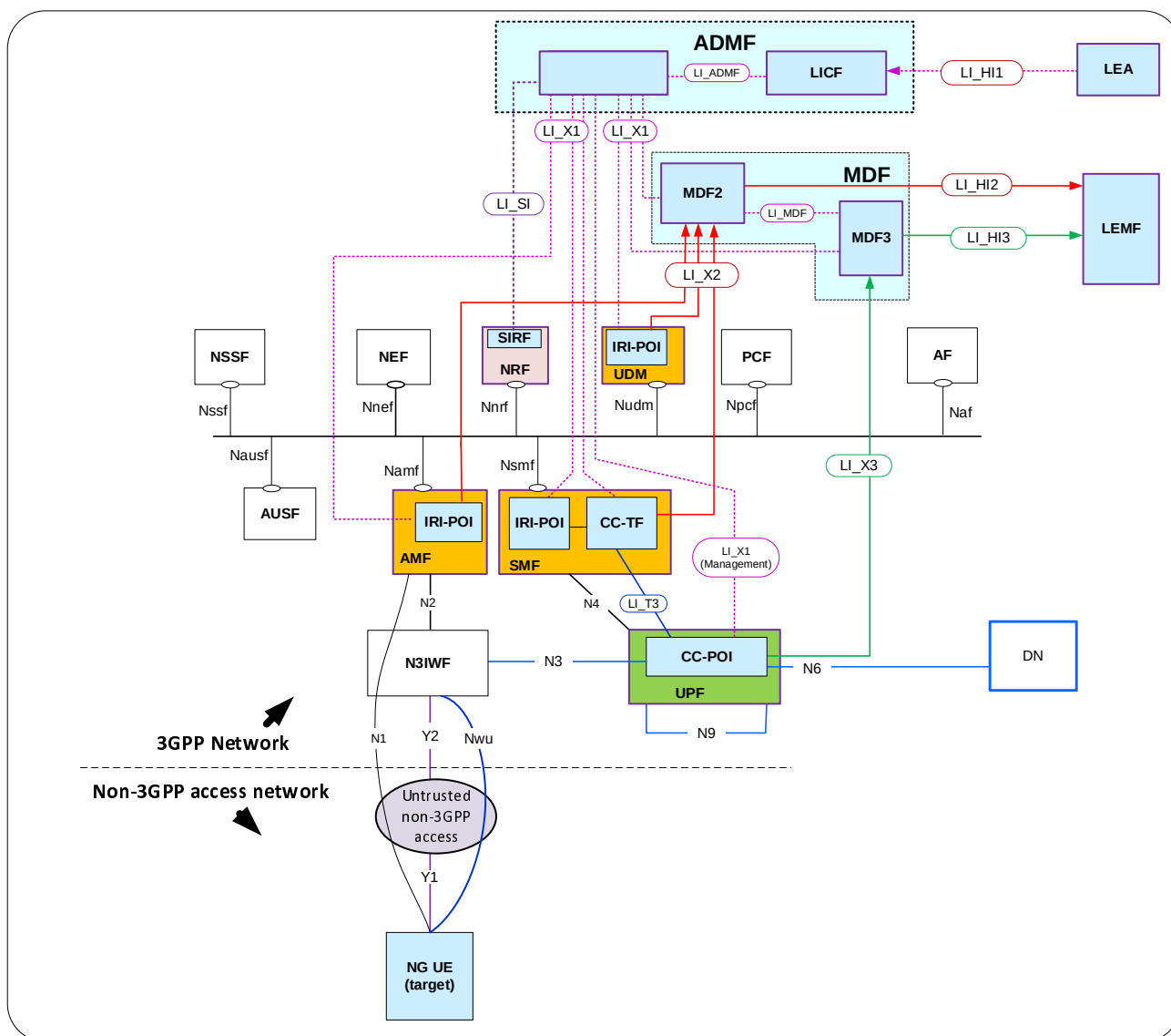
Figure A.4.2-1: Network topology showing LI for non-3GPP access to 5G via N3IWF
