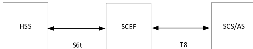
Figure 7.11.5.1-1: EPS architecture for Parameter Provisioning
