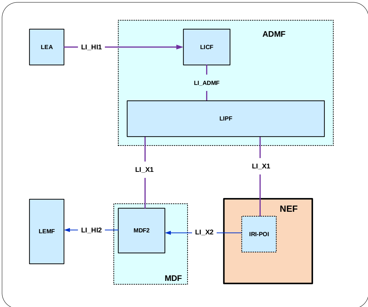
Figure 7.9.3.2-1: LI architecture for device triggering using NEF
