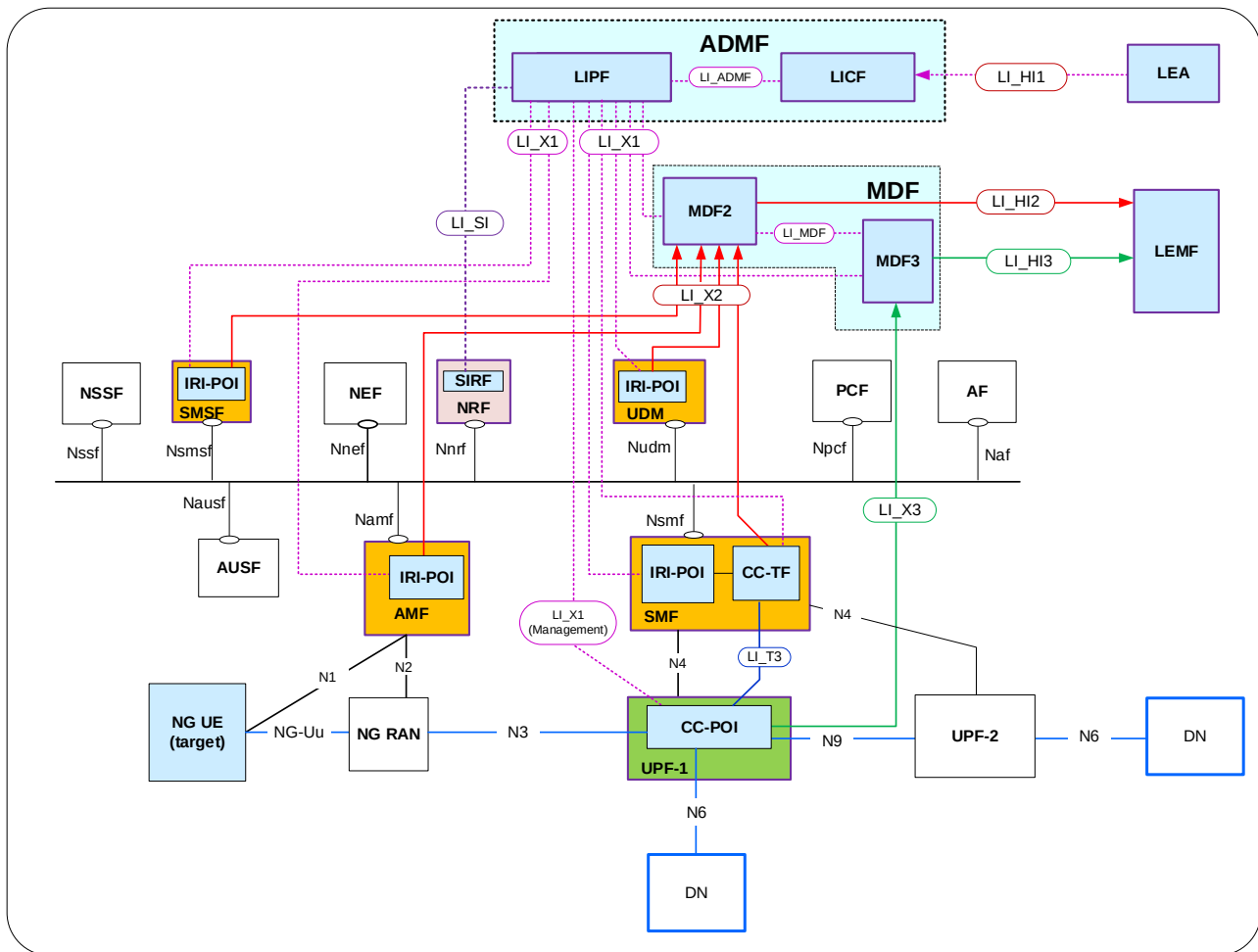
Figure A.3.2-1: Network topology showing CC-POI at one UPF
