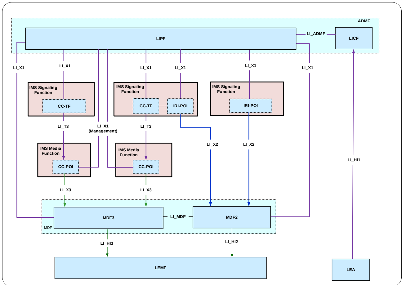
Figure 7.4.2.1-1: IMS LI architecture
