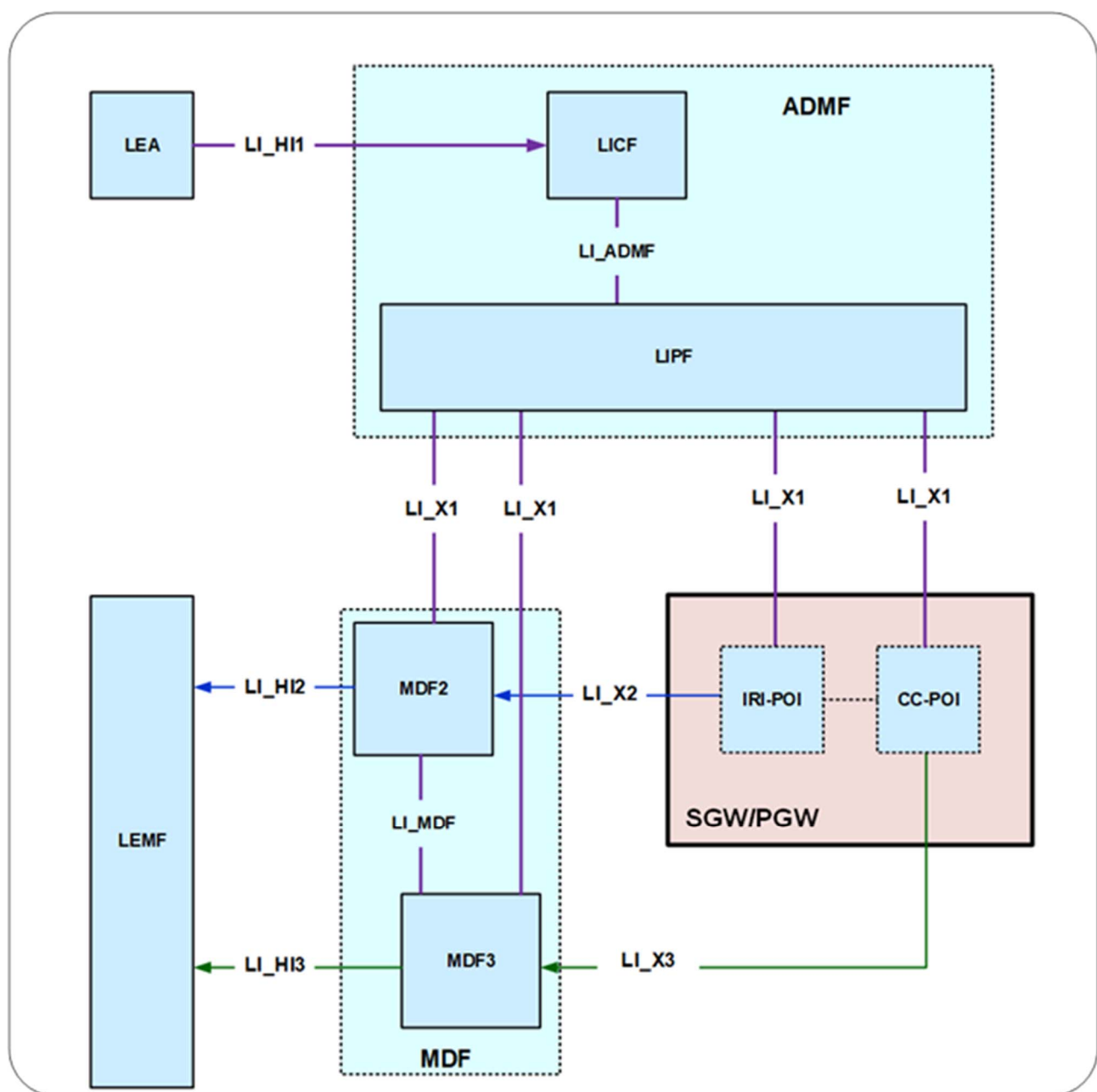
Figure 6.3.3.1.2-1: LI architecture for LI at non-CUPS SGW/PGW
