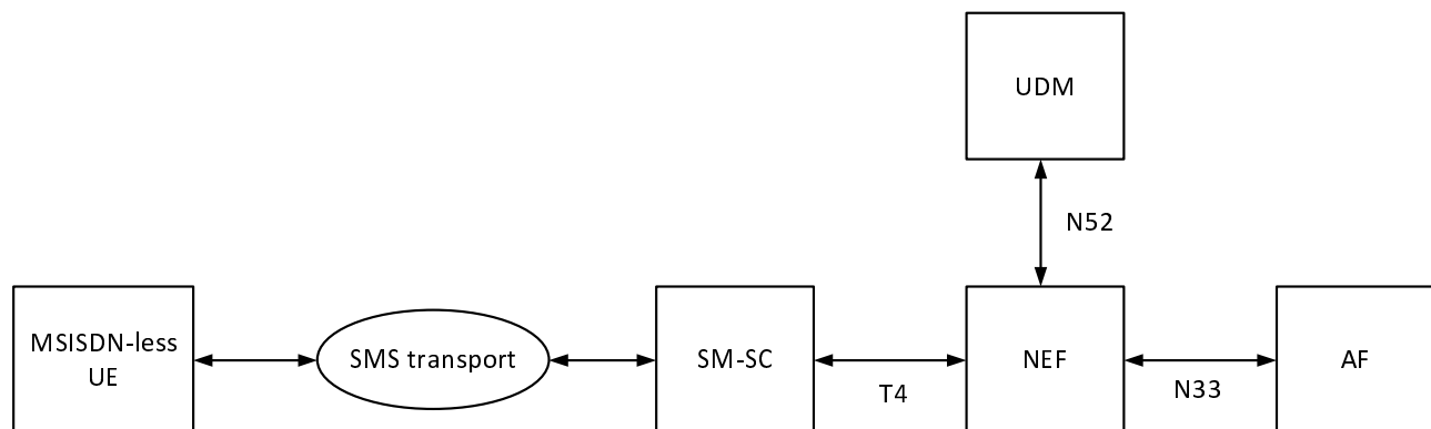
Figure 7.9.4.1-1: 5GS architecture for MSISDN-less MO SMS
