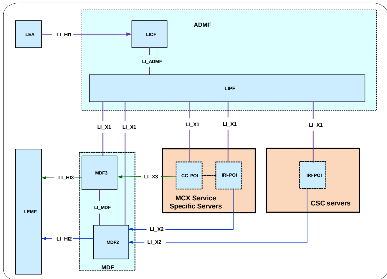
Figure 7.23.2-1: LI architecture for Mission Critical Services
