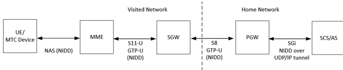
Figure 7.10.1.3.2-1: EPS Architecture for NIDD using a PtP SGi tunnel in roaming situation
