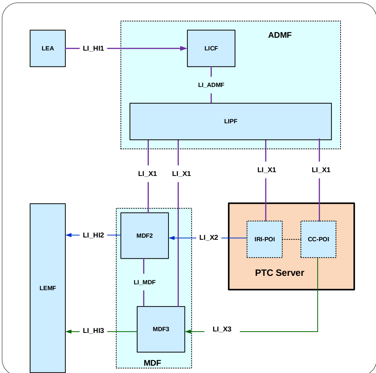
Figure 7.6.1.2-1: LI architecture for PTC
