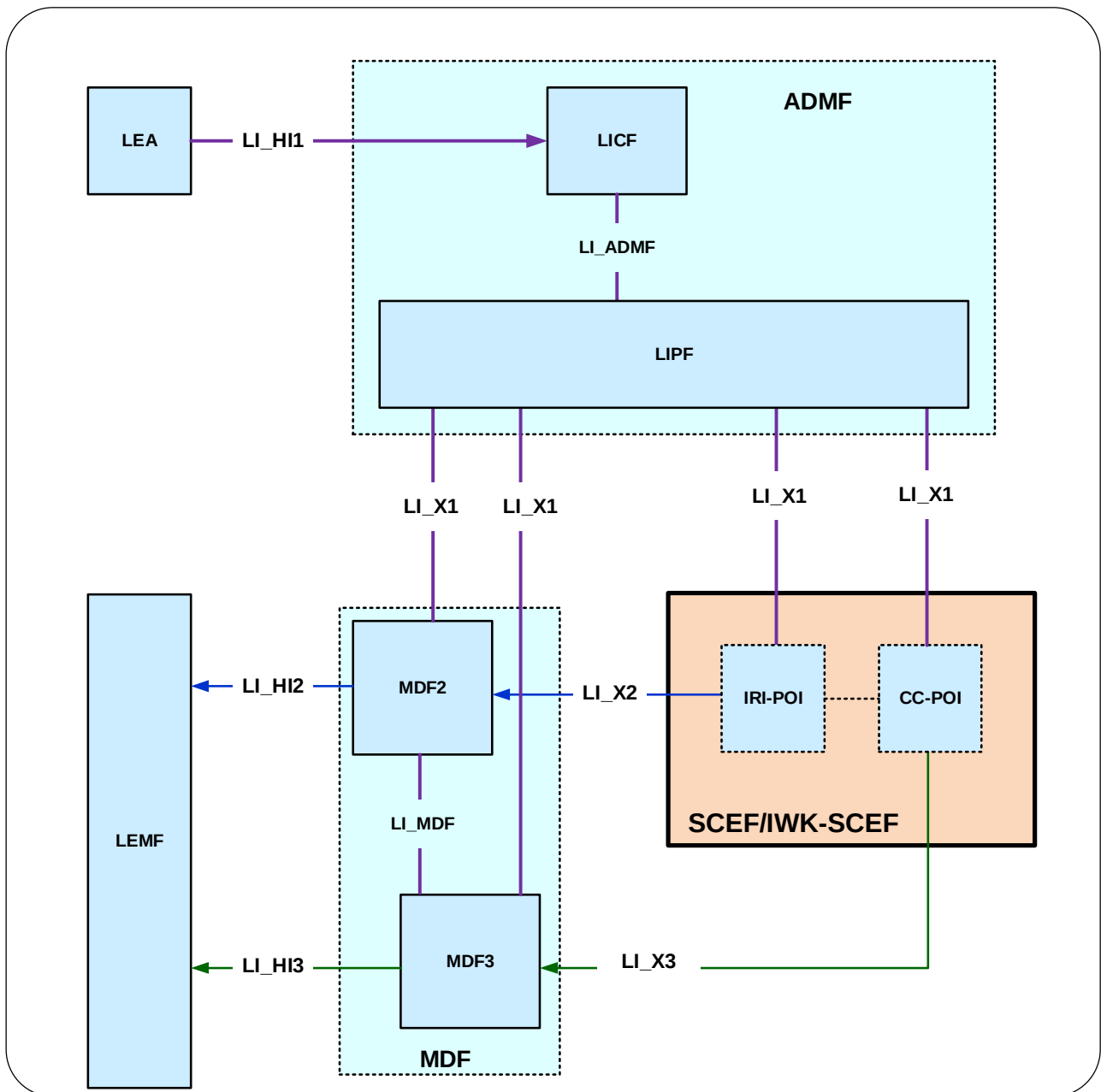
Figure 7.11.2.1-1: LI architecture for NIDD using SCEF showing LI at SCEF/IWK-SCEF
