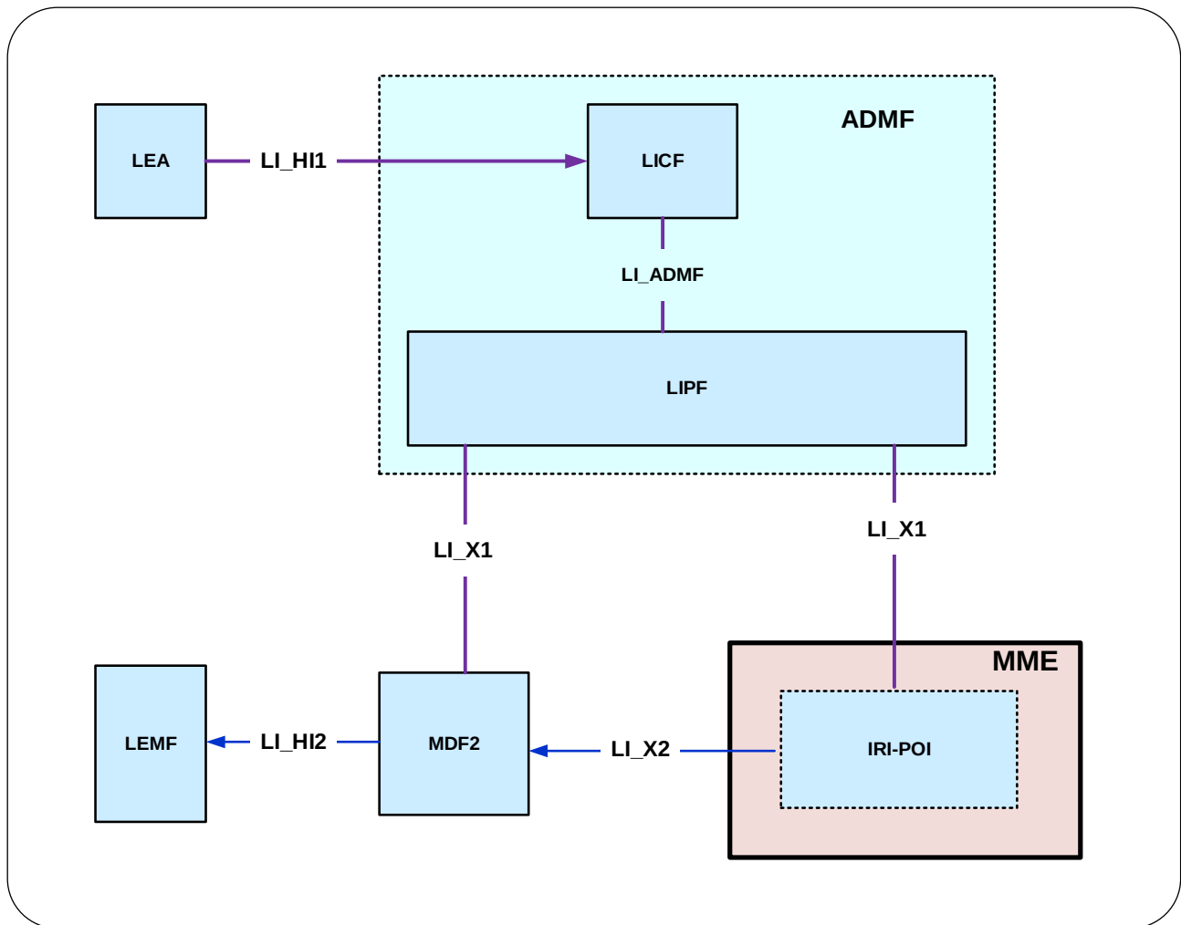
Figure 6.3.2.1-1: LI architecture for LI at MME
