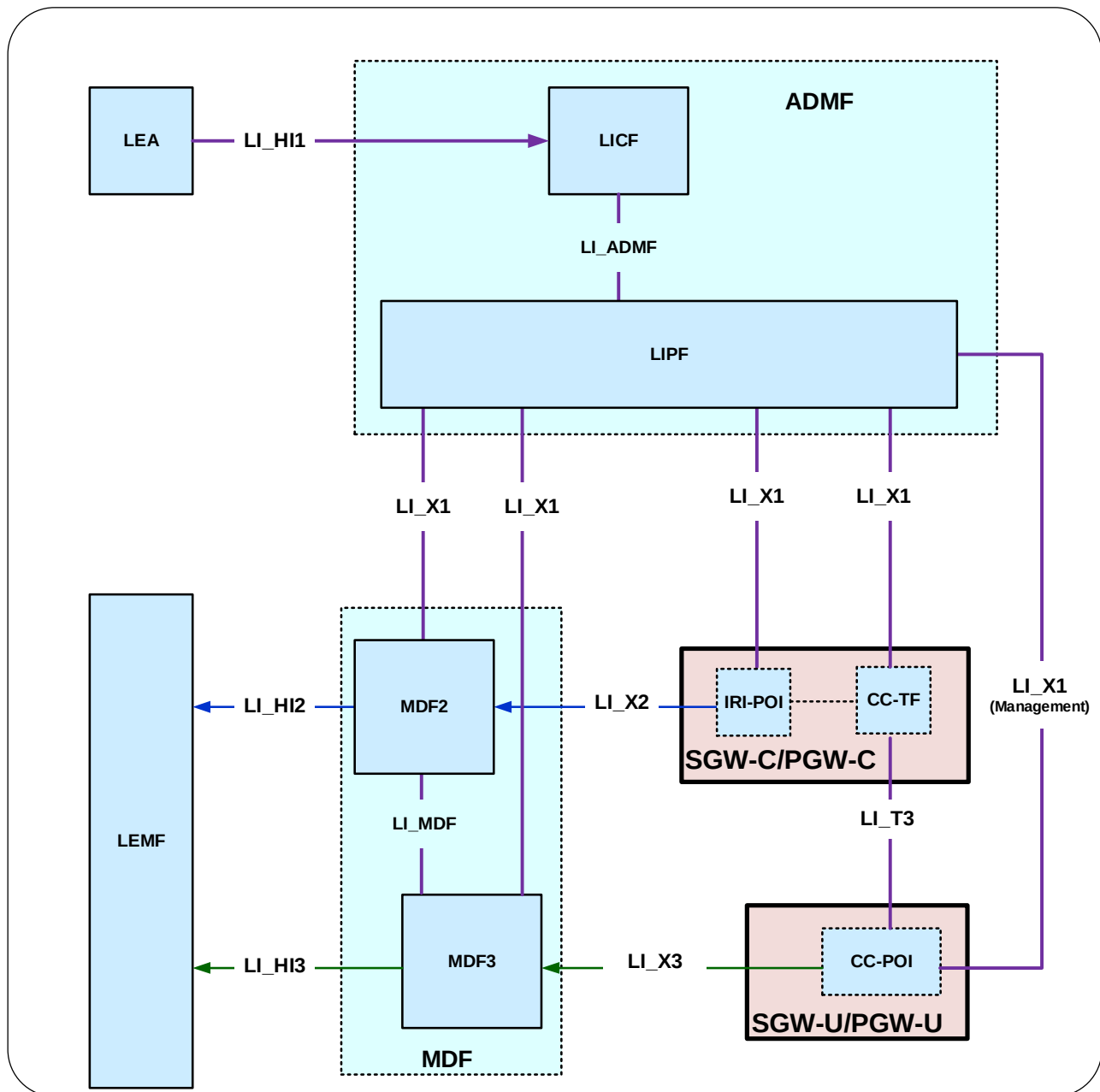
Figure 6.3.3.1.3-1: LI architecture for LI at EPS CUPS SGW/PGW
