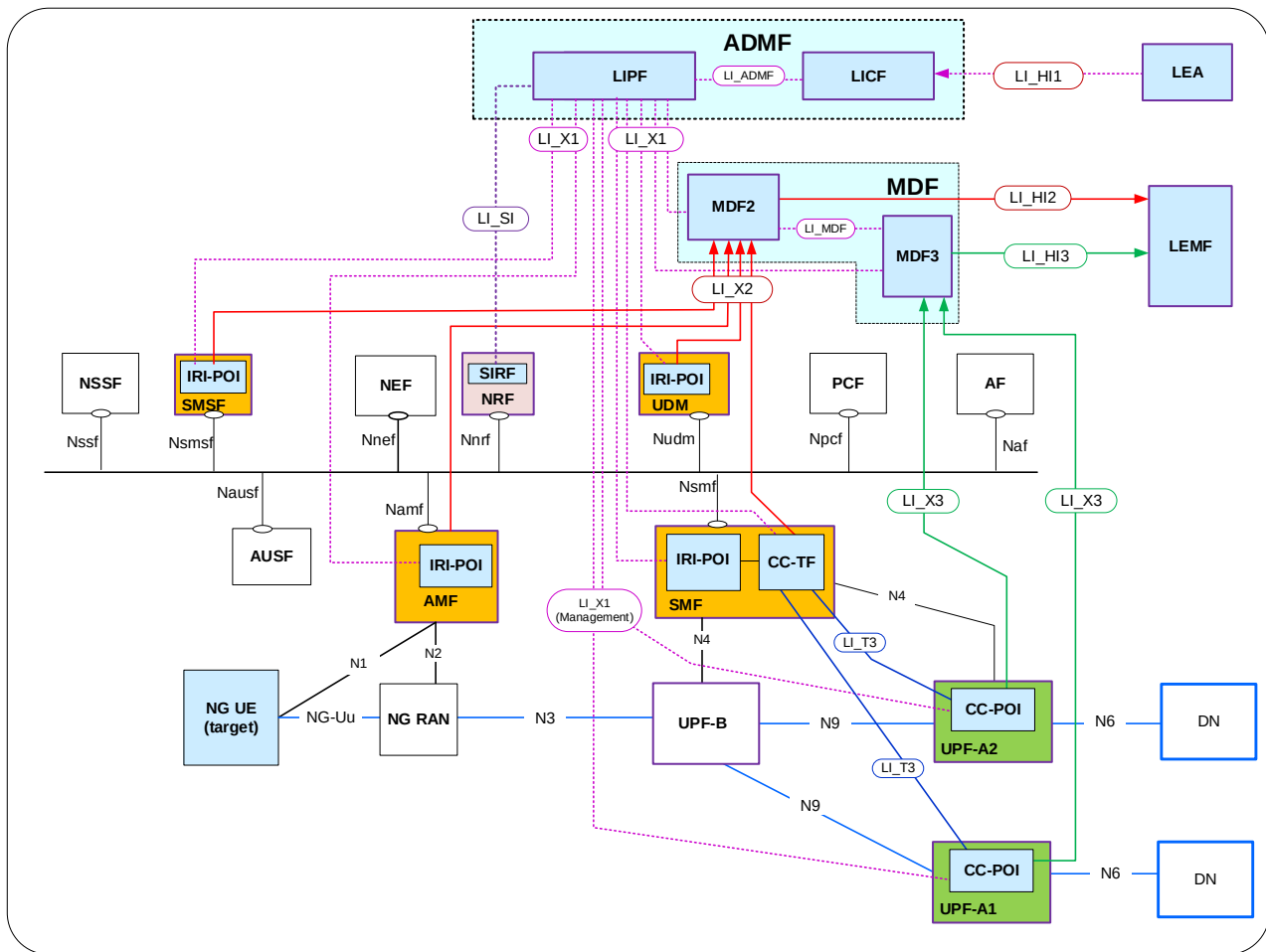
Figure A.3.2-2: Network topology showing CC-POI at two UPFs
