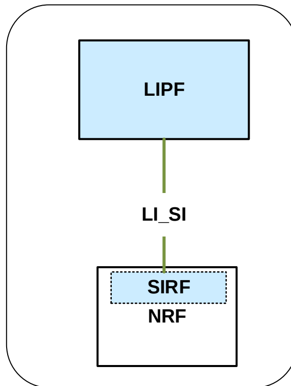
Figure 6.2.6.1-1: LI Architecture depicting NRF as an SIRF
