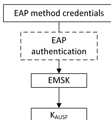
Figure 1.2.3.1-1: K_{AUSF} derivation for key-generating EAP authentication methods other than EAP-AKA'
