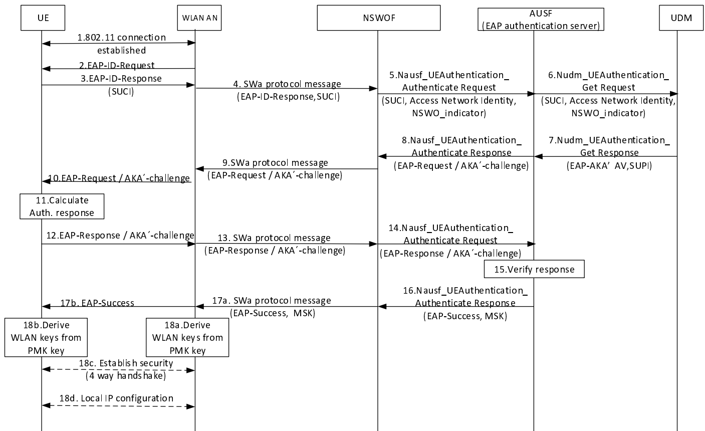
Figure: S.3-1: Authentication procedure for NSWO in 5G
