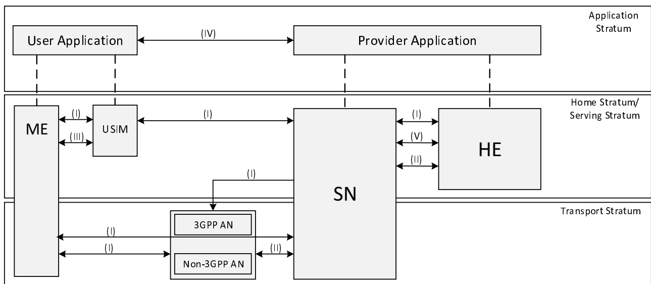
Figure 4-1: Overview of the security architecture
