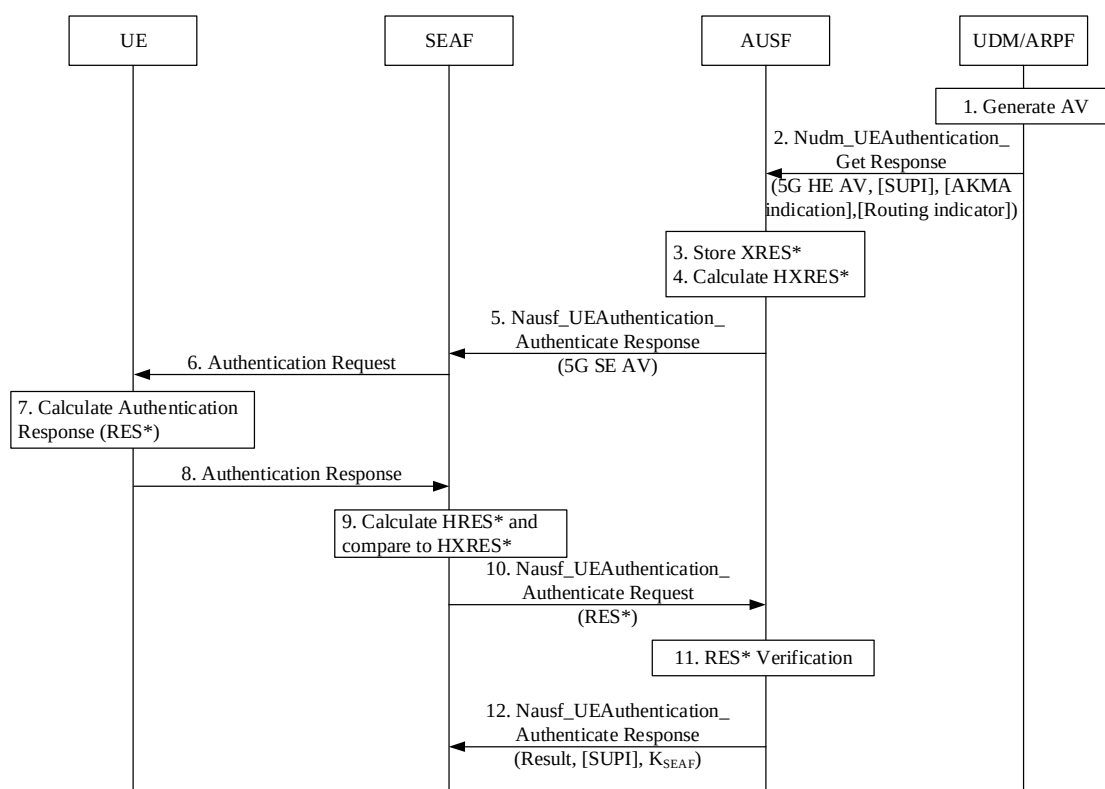
Figure 6.1.3.2-1: Authentication procedure for 5G AKA
