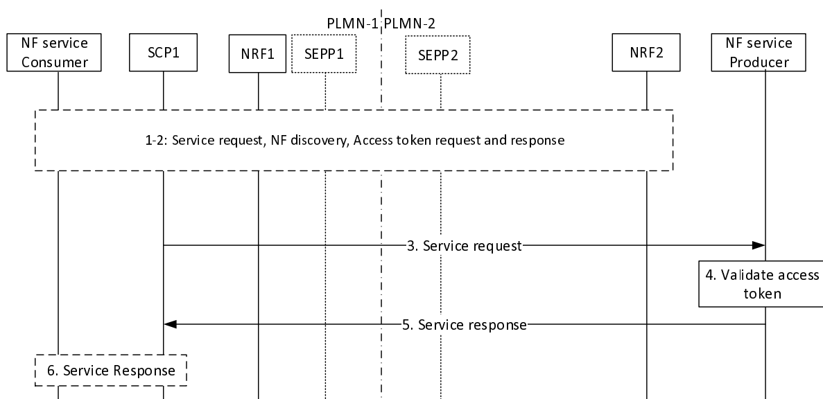
Figure 13.4.1.5.2.2-1: Service access authorization in indirect communication (with or without delegated discovery) when NF Service Consumer and NF Service Producer are in different PLMNs and NF selection is at the source PLMN
