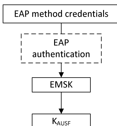
Figure I.2.3.1-1: K_{AUSF} derivation for key-generating EAP authentication methods other than EAP-AKA'
