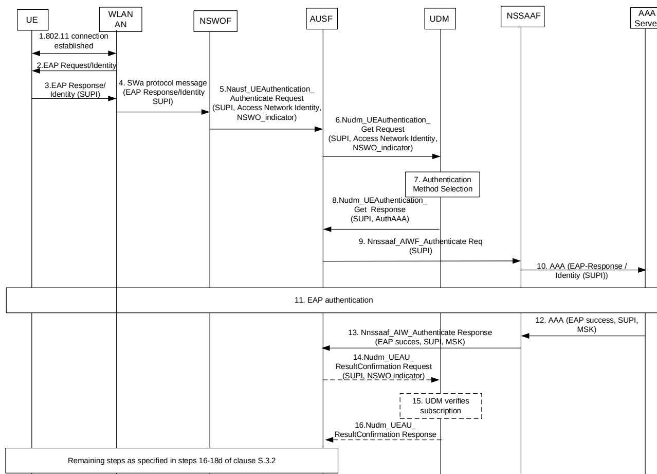
Figure I.10.5.1.2-1 - Procedure for NSWO authentication using CH with AAA server via 5GC
