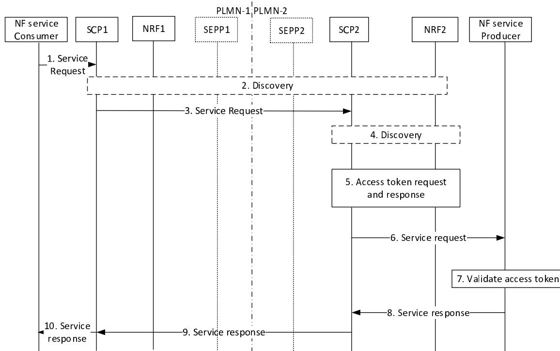
Figure 13.4.1.5.3.3-1: Service access authorization when NF Service Consumer and NF Service Producer are in different PLMNs with indirect communication with delegated discovery and NF selection is at target PLMN
