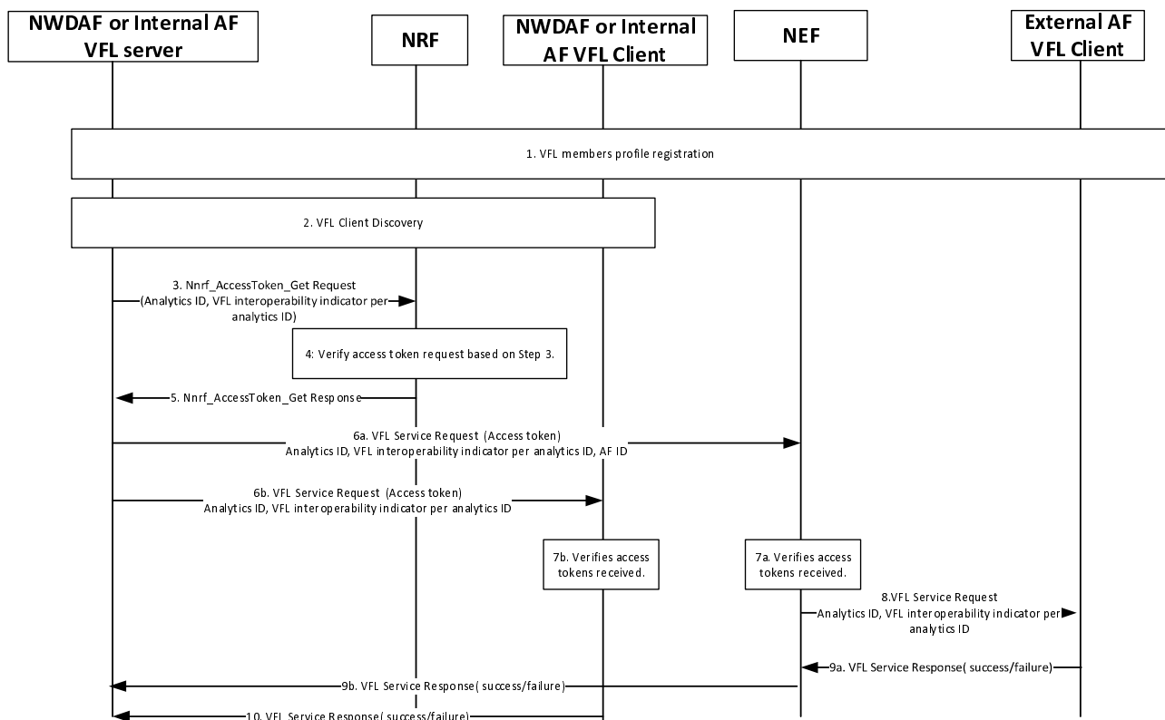
Figure X.12.2.1-1: Authorization of VFL participants (NWDAF or Internal AF acts as VFL Server)
