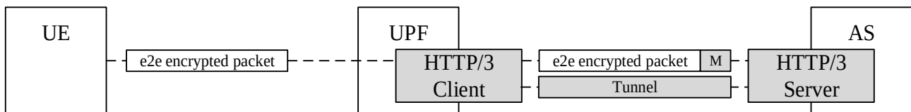
Figure 18.2.3-1: Overview of the connect-UDP Forward mode architecture for protection of XRM Media related information
