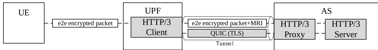
Figure 18.2.1-1: Overview of the connect-UDP Tunnelling mode architecture for protection of XRM Media related information
