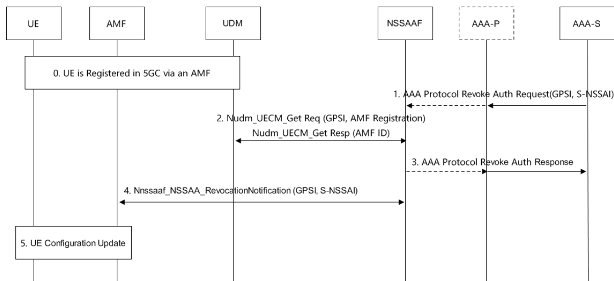
Figure 16.5-1: AAA Server-initiated Network Slice-Specific Authorization Revocation procedure
