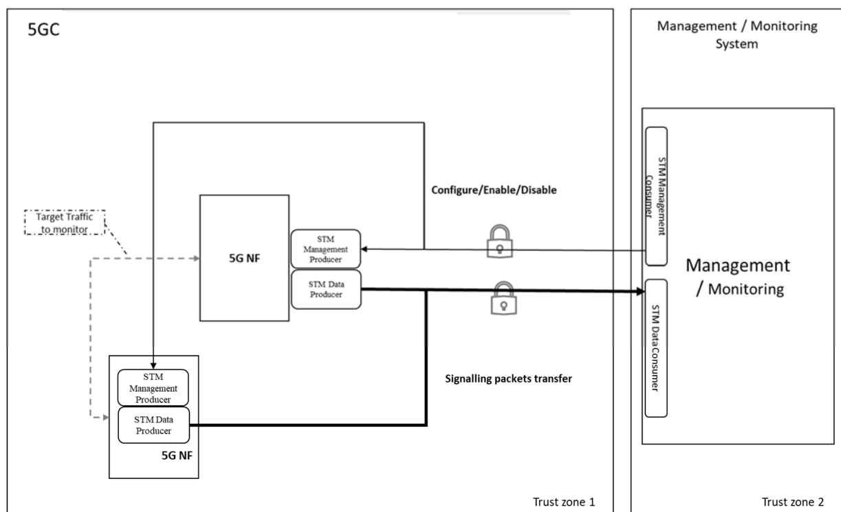
Figure 17.1-1 Signalling Traffic Monitor trust zones example
