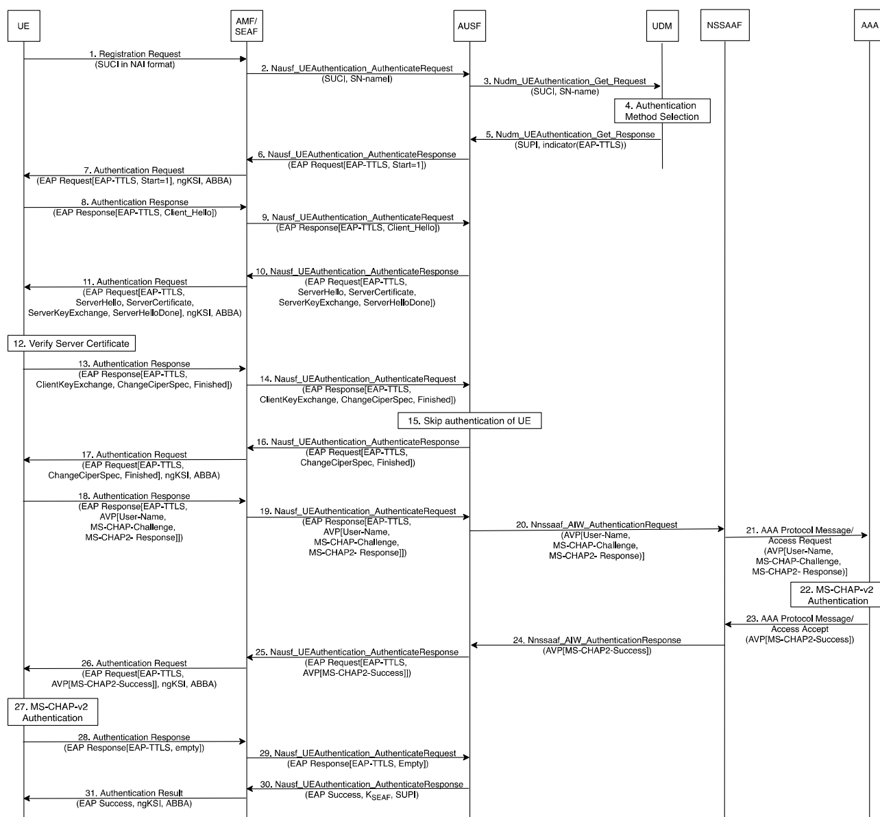
Figure: U.2-1: Primary authentication using EAP-TTLS and AAA
