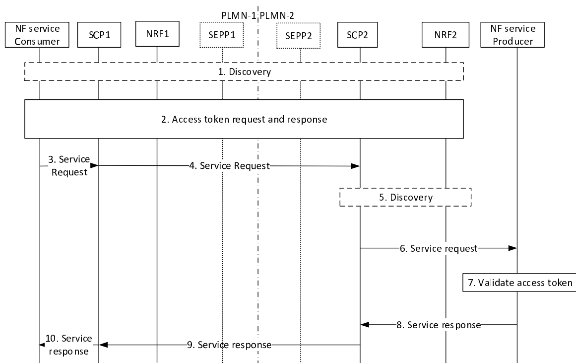
Figure 13.4.1.5.3.2-1: Service access authorization when NF Service Consumer and NF Service Producer are in different PLMNs with indirect communication without delegated discovery and NF selection is at target PLMN
