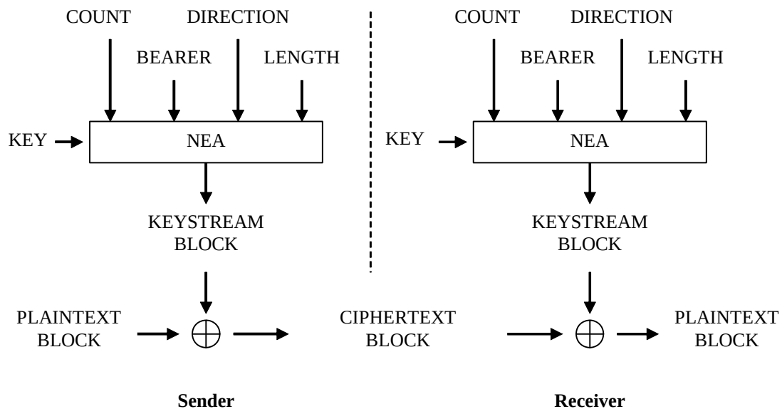
Figure D.2.1.1-1: Ciphering of data
