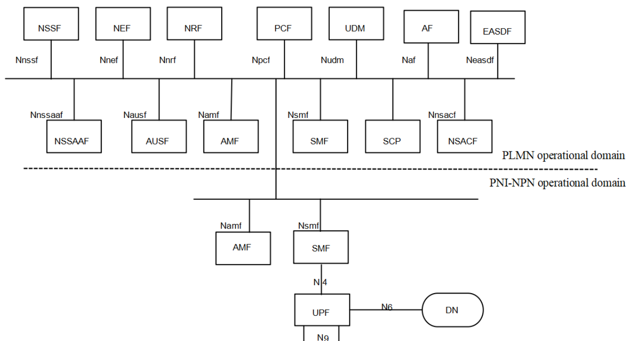
Figure AB.2-1 Example of dedicated NFs deployed in the PNI-NPN operational domain
