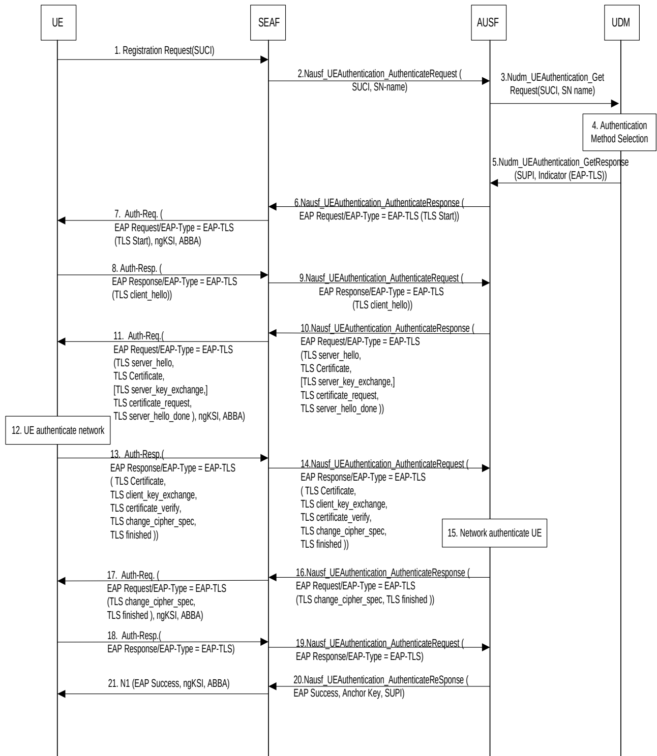
Figure B.2.1.1-1: Using EAP-TLS 1.2 Authentication Procedures over 5G Networks for initial authentication
