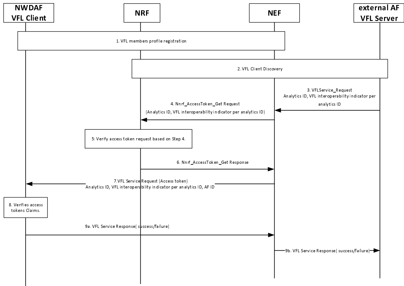
Figure X.12.2.2-1: Authorization of candidate VFL participants for VFL when external AF is acting as the VFL server
