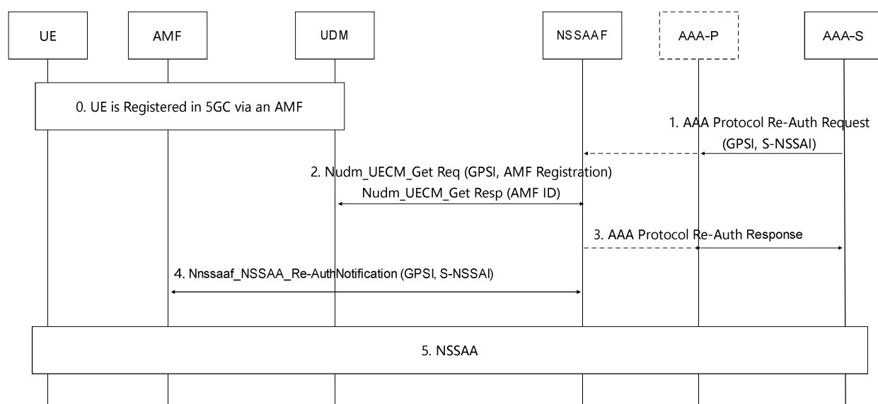
Figure 16.4-1: AAA Server initiated Network Slice-Specific Re-authentication and Re-authorization procedure
