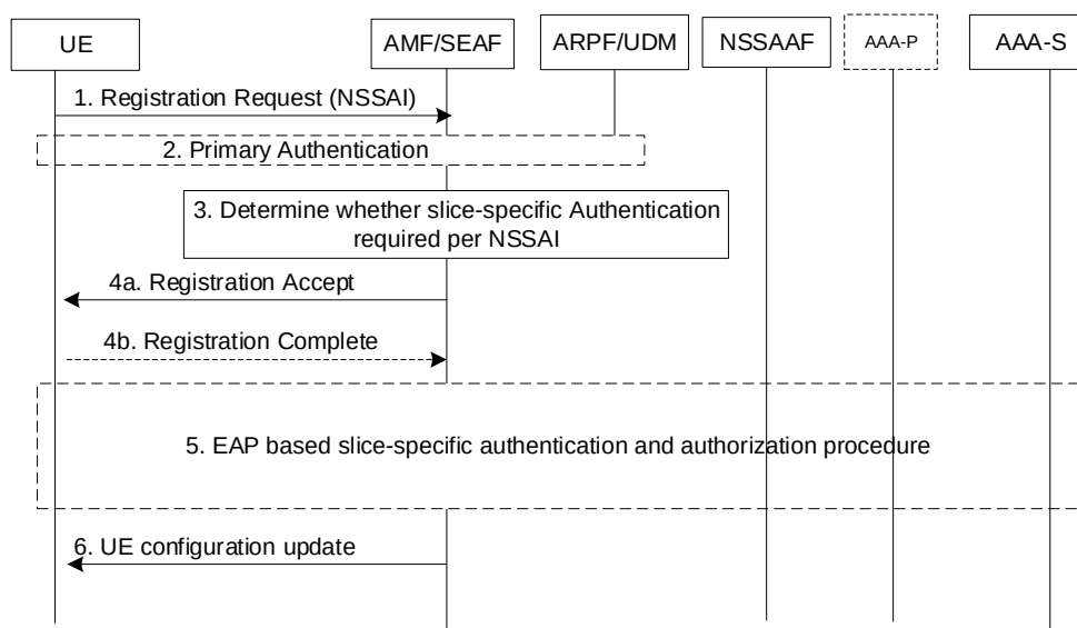
Figure 16.2-1: Relationship between primary authentication and NSSAA
