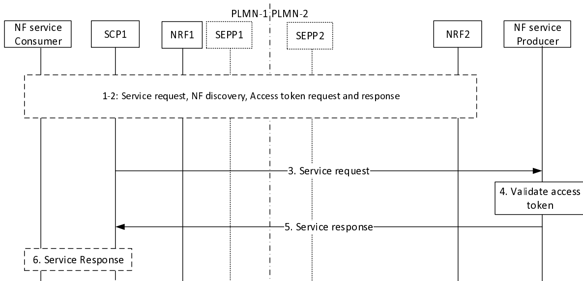
Figure 13.4.1.5.2.2-1: Service access authorization in indirect communication (with or without delegated discovery) when NF Service Consumer and NF Service Producer are in different PLMNs and NF selection is at the source PLMN
