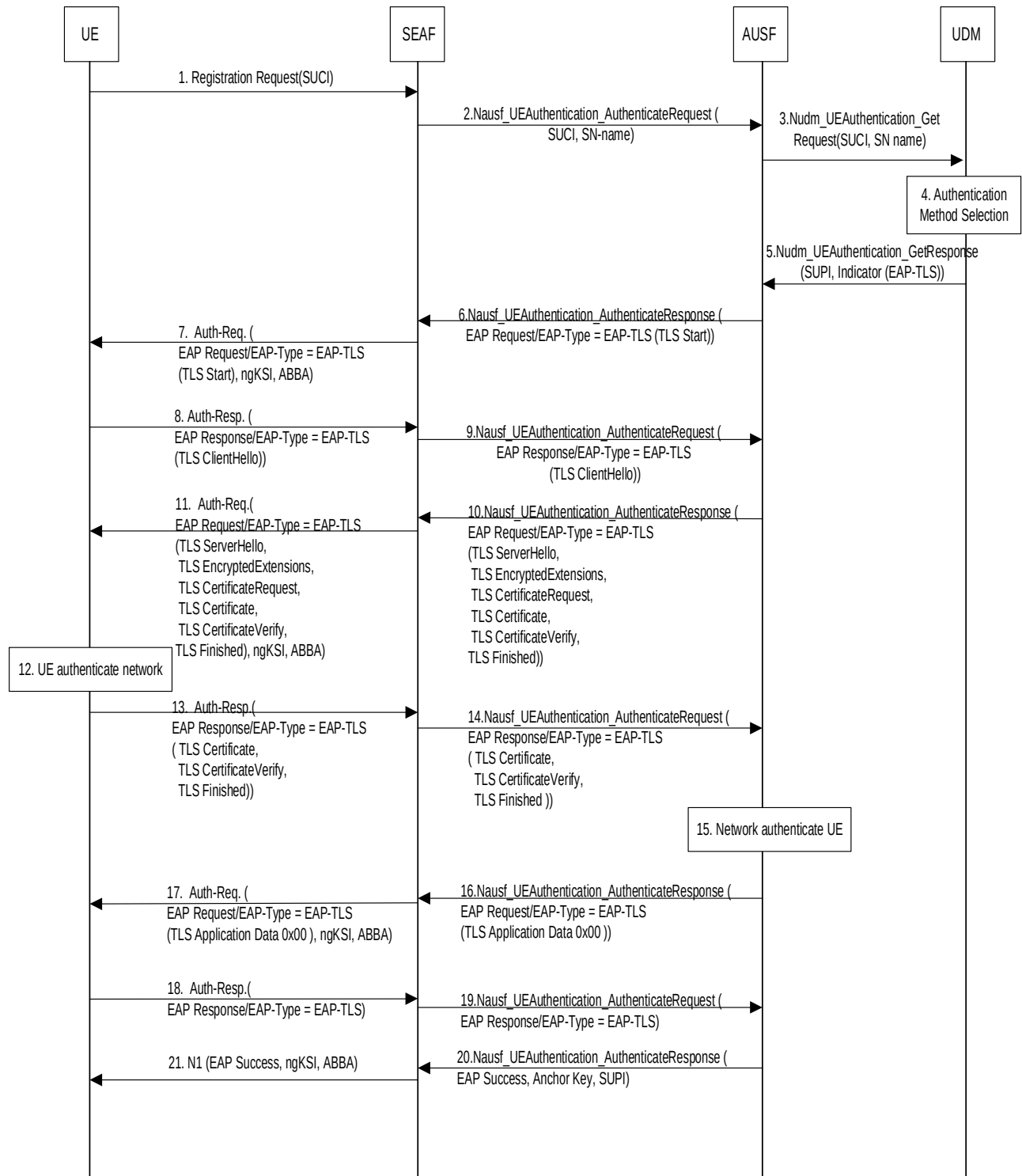
Figure B.2.1.1-2: Using EAP-TLS 1.3 Authentication Procedures over 5G Networks for initial authentication
