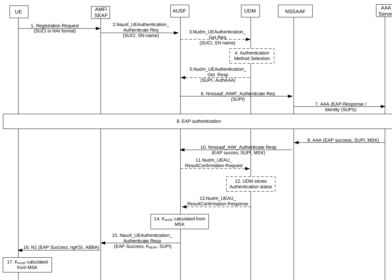
Figure: 1.2.2.2.2-1: Primary authentication with external domain
