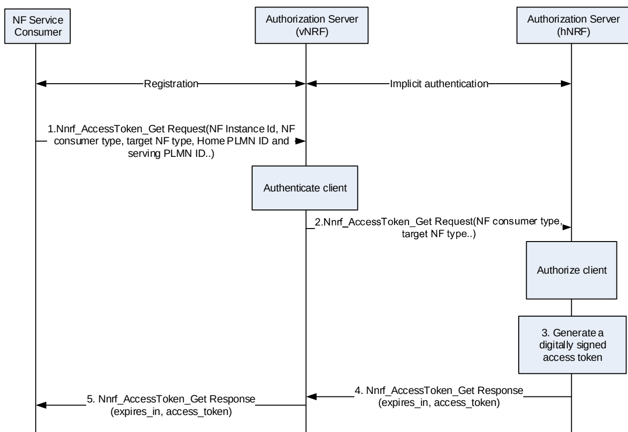
Figure 13.4.1.2.2-1: NF Service Consumer obtaining access token before NF Service access (roaming)
