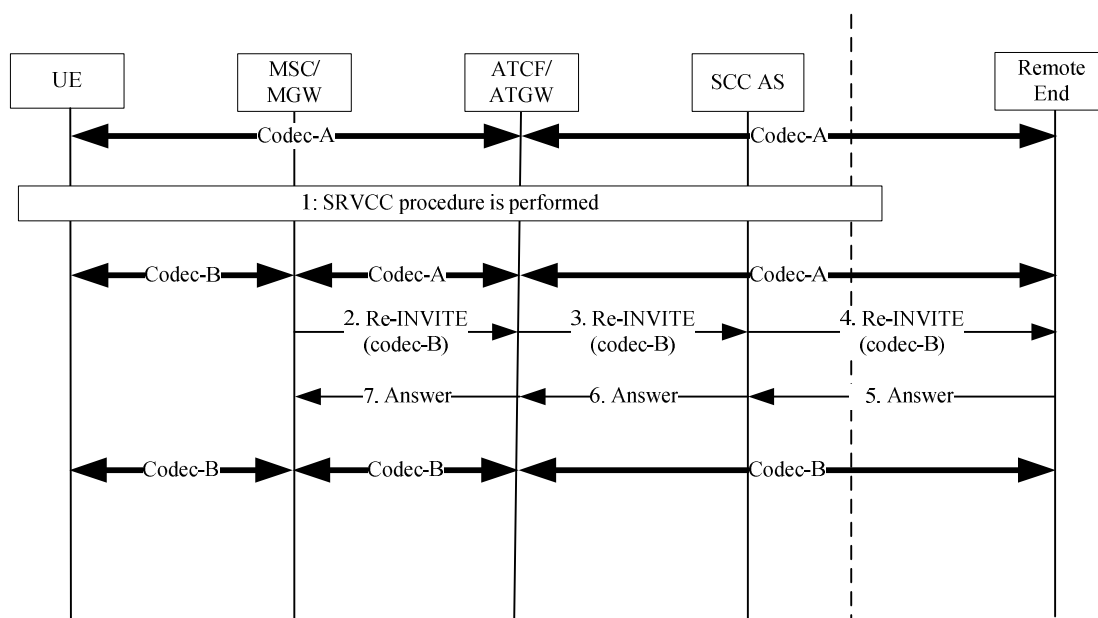
Figure B.2.1-1: Re-negotiation method towards the remote end
