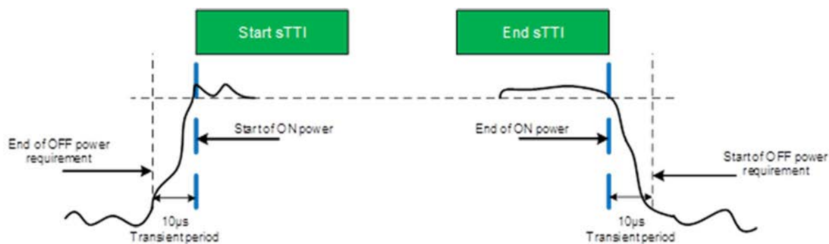
Figure 6.3.4.1-1B: General ON/OFF time mask for sTTI and for Frame Structure Type 1 and Frame Structure Type 2
