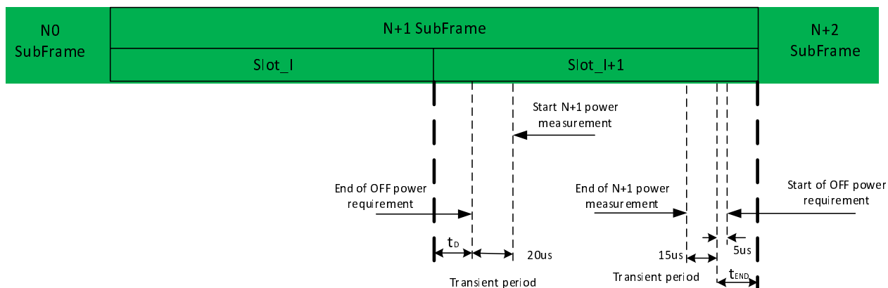
Figure 6.3.4.3-1C: Transmission power template for the second slot in one subframe for Frame Structure Type 3
