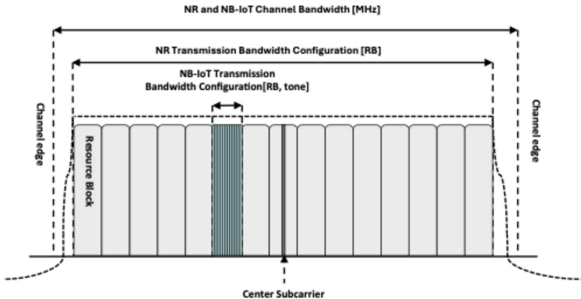
Figure 5.3B-2 Definition of Channel Bandwidth and Transmission Bandwidth Configuration for NB-IoT operation in NTN NR in-band
