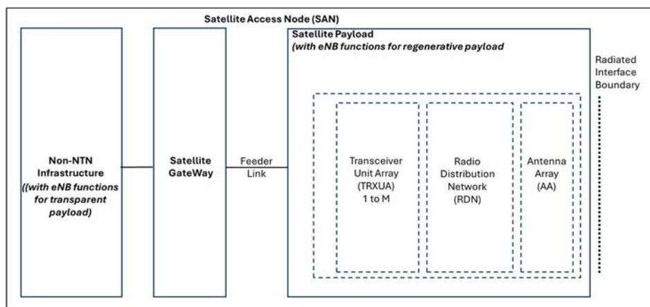
Figure 4.3.2-1: Radiated reference points for SAN type 1-O
