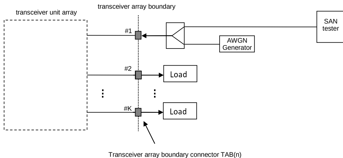
Figure D.5.2-1: Functional set-up for performance requirements for PUSCH and PRACH in static conditions for SAN with 1Rx case shown
