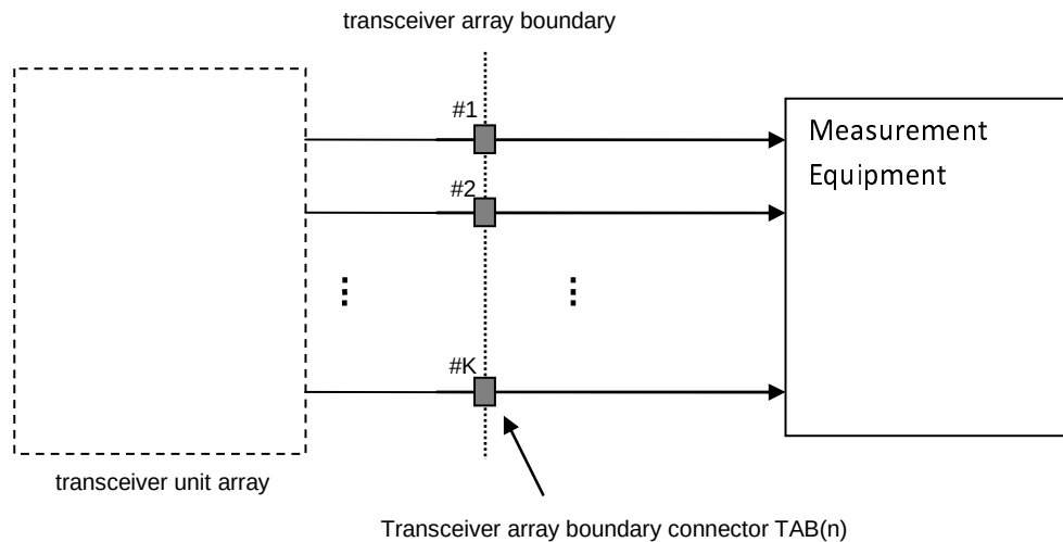
Figure D.1.1-2: Measuring system set-up for SAN type 1-H output power, output power dynamics, frequency error, EVM, unwanted emissions for multiple TAB connectors
