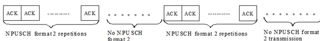
Figure 11.5.2.4.2-1: Test signal pattern for NPUSCH format 2 demodulation tests
