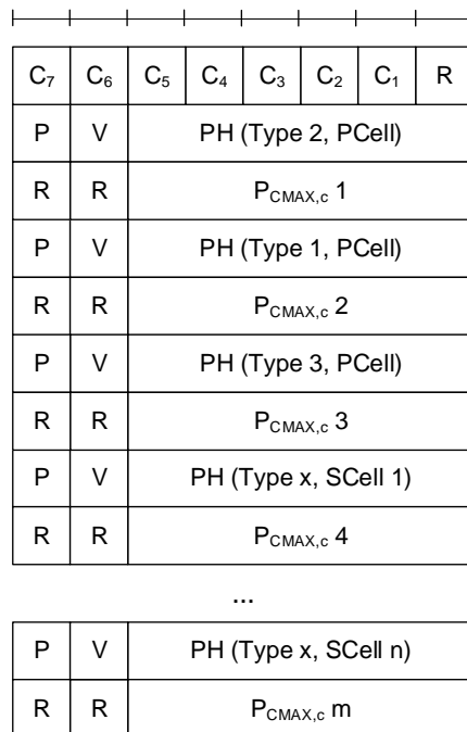
Figure 6.1.3.6a-2: Extended PHR MAC Control Element
