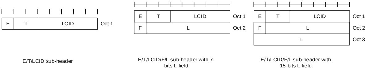
Figure 6.1.7-3: E/T/LCID/(F)/(L) MAC subheader
