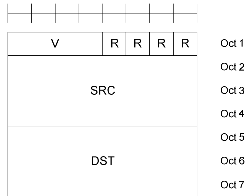
Figure 6.1.6-3a: SL-SCH MAC subheader for V="0011"
