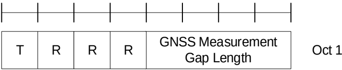
Figure 6.1.3.22-1: GNSS Measurement Command MAC control element
