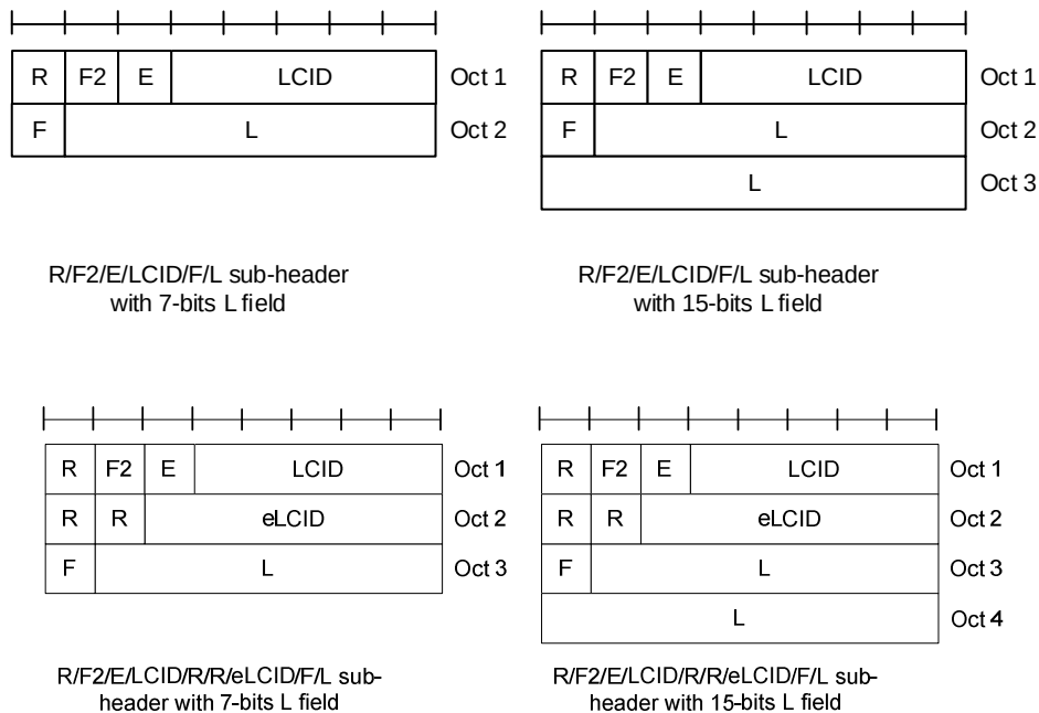
Figure 6.1.2-1: R/F2/E/LCID/(R/R/eLCID)/F/L MAC subheader with 7-bits and 15-bits L field
