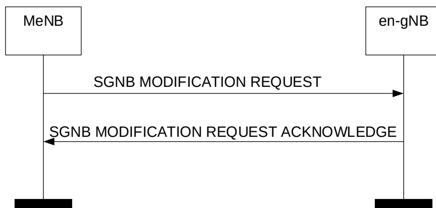
Figure 8.7.6.2-1: MeNB initiated SgNB Modification Preparation, successful operation
