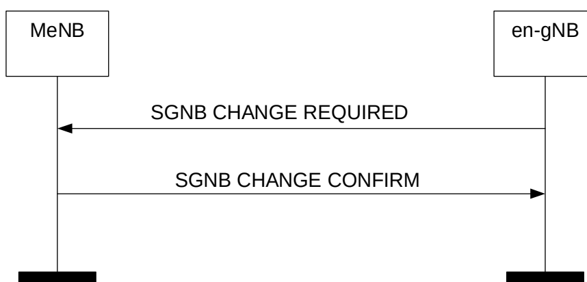
Figure 8.7.8.2-1: SgNB Change, successful operation.
