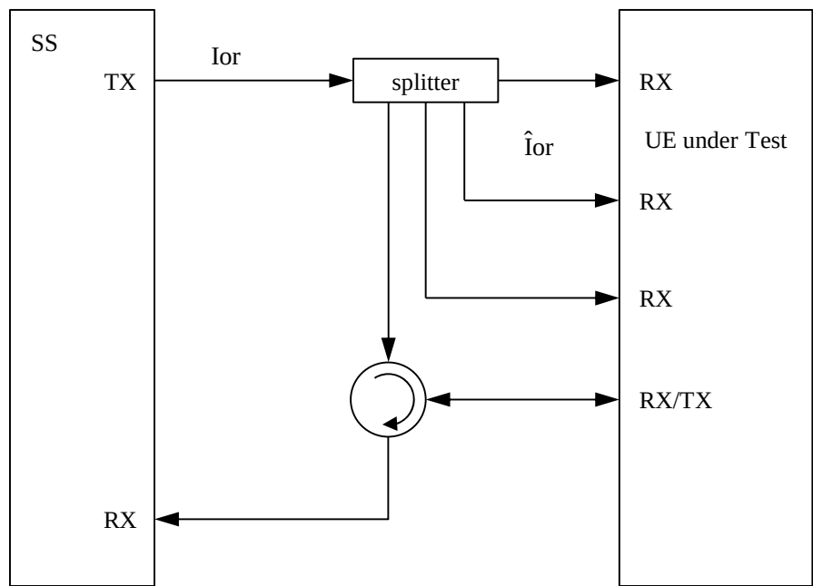
Figure A.69: Connection for Receiver test with 4 Rx antenna ports
