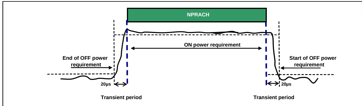
Figure 6.3B.3.2.3-1: NPRACH ON/OFF time mask
