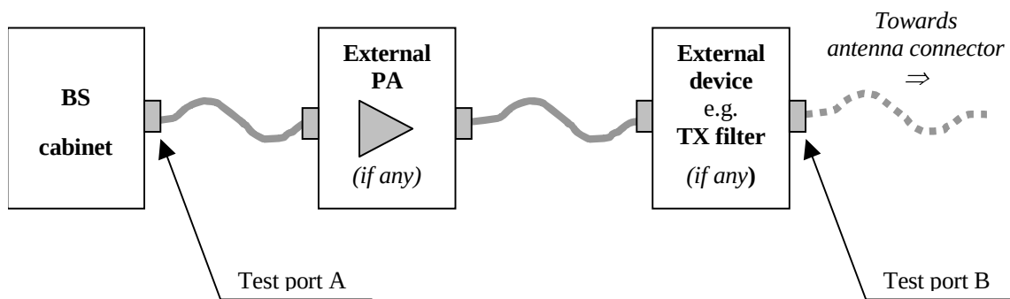
Figure 4.10.1-1: Transmitter test ports
