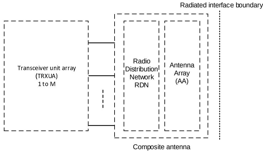
Figure 4.2-2: Radiated points of reference of OTA AAS BS
