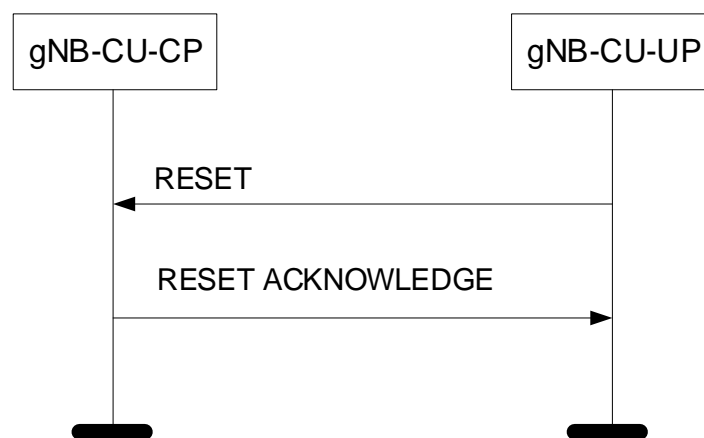
Figure 8.2.1.2.2-1: Reset procedure initiated from the gNB-CU-UP. Successful operation.
