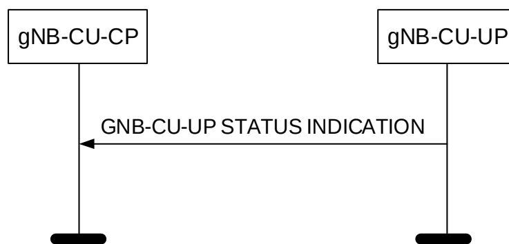
Figure 8.2.8.2-1: gNB-CU-UP Status Indication procedure: Successful Operation.
